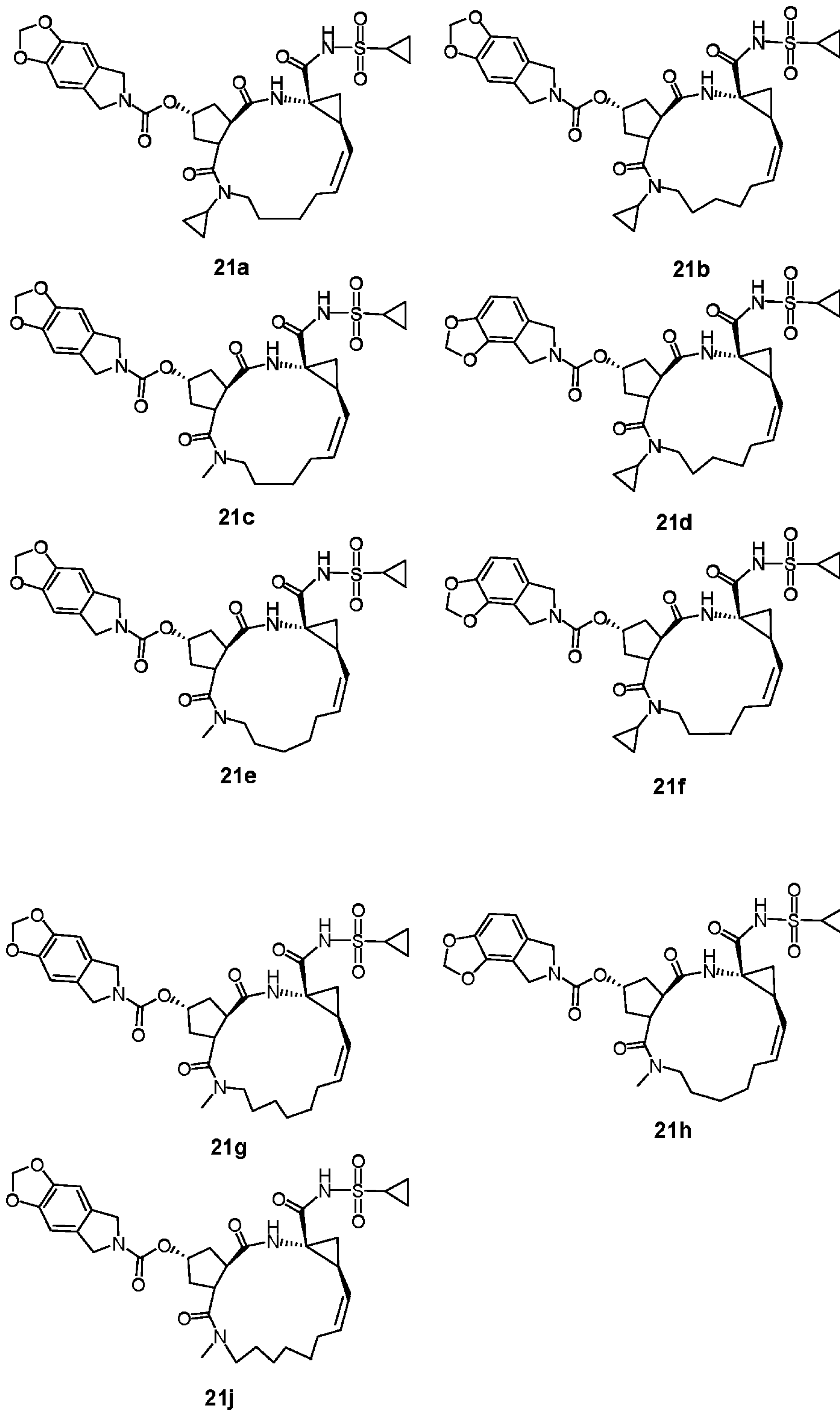
Figure 7: Structure of Compounds 21a-21j
