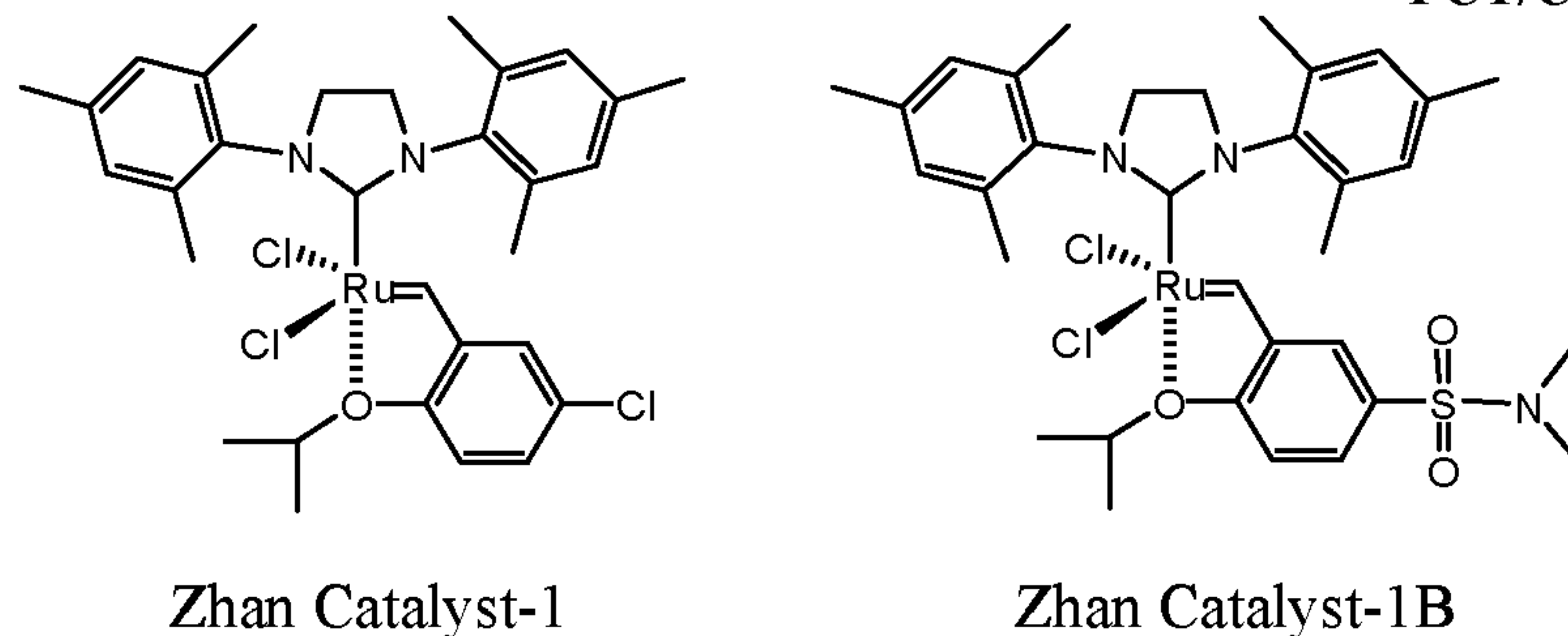
Figure 3: Structure of Zhan catalyst-1 and Zhan Catalyst-1B
