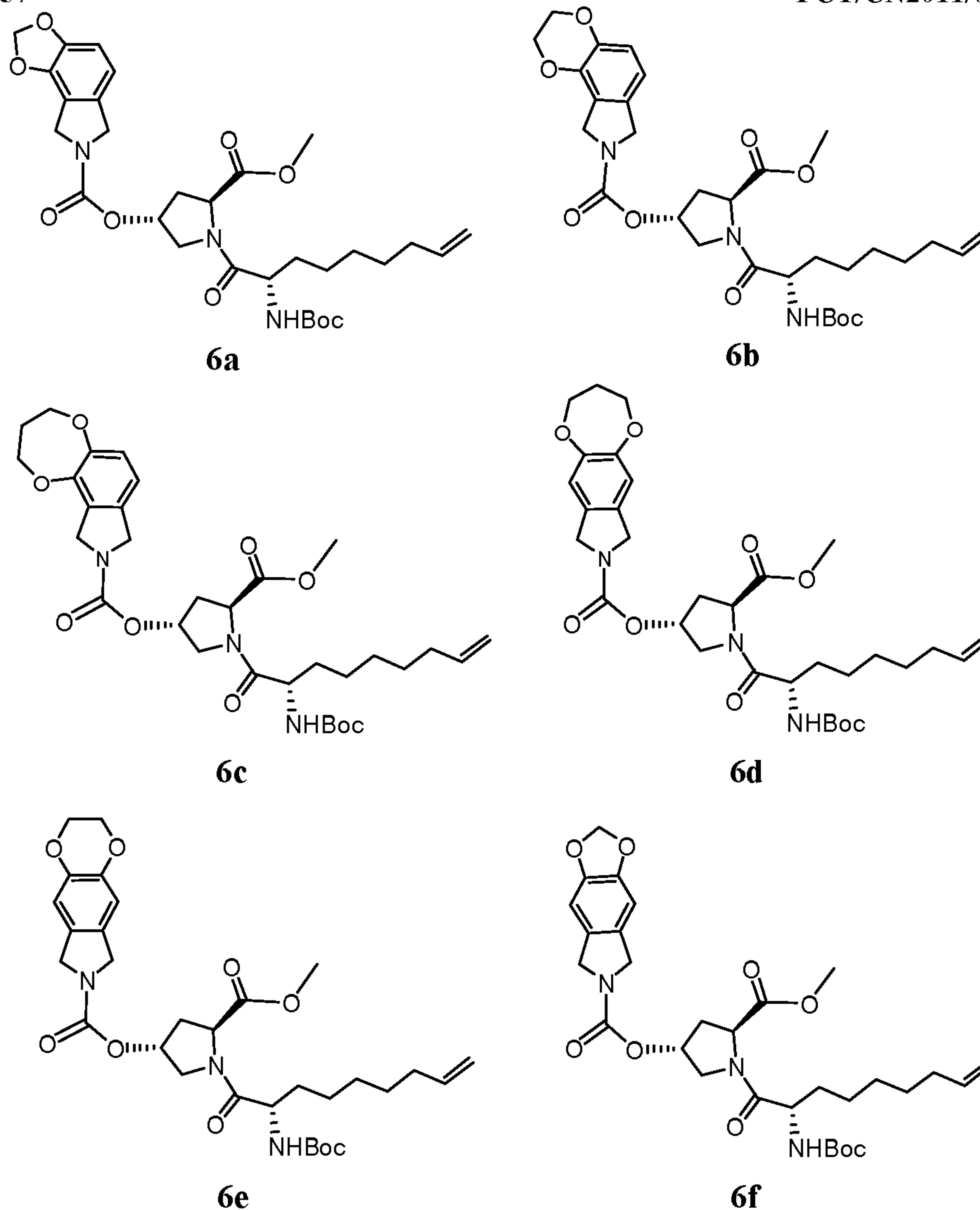
Figure 1-2: Structure of Compounds 6a-6f
