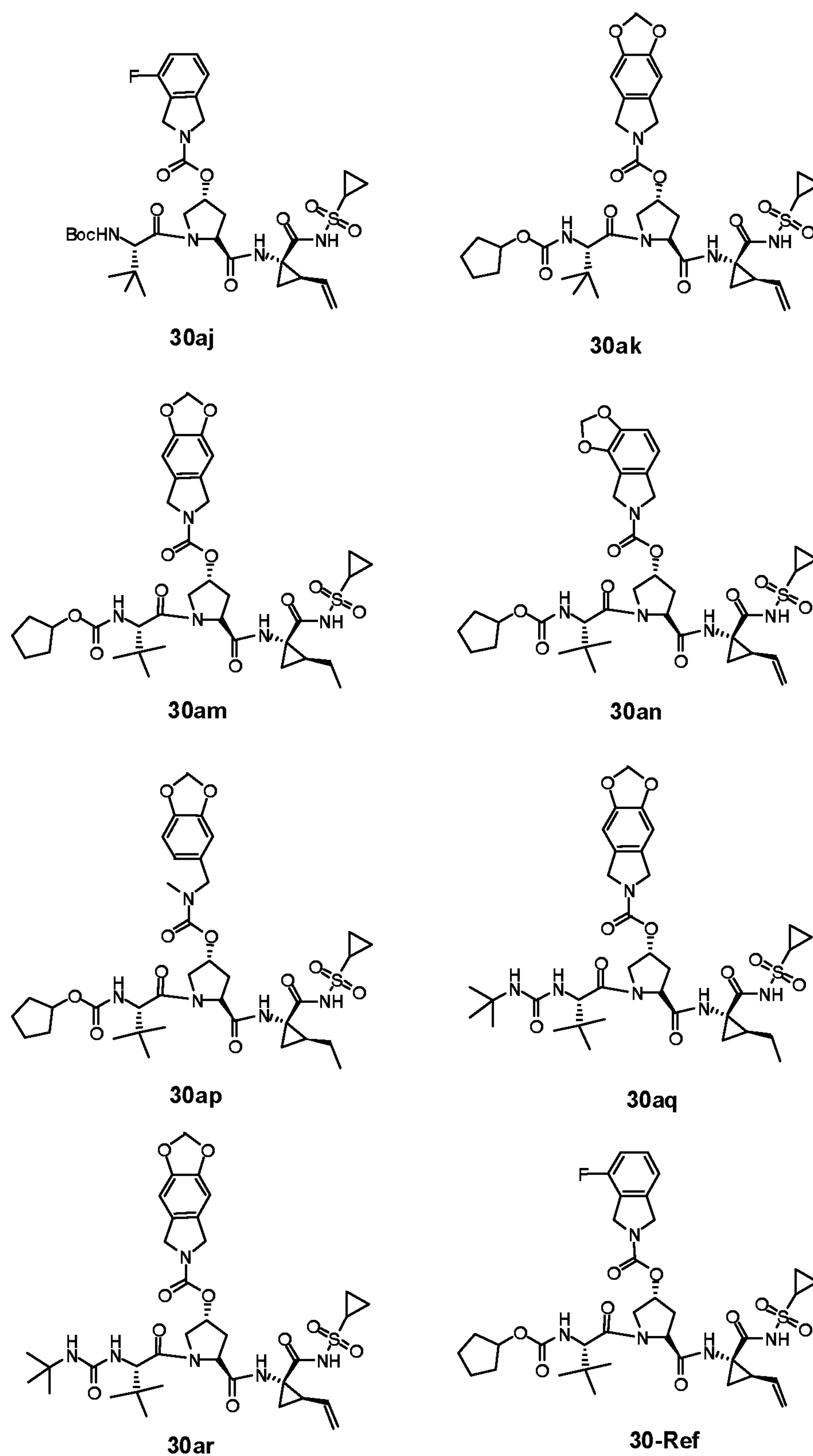
Figure 10: Structure of Compounds 30a-30ar and 30-Ref
