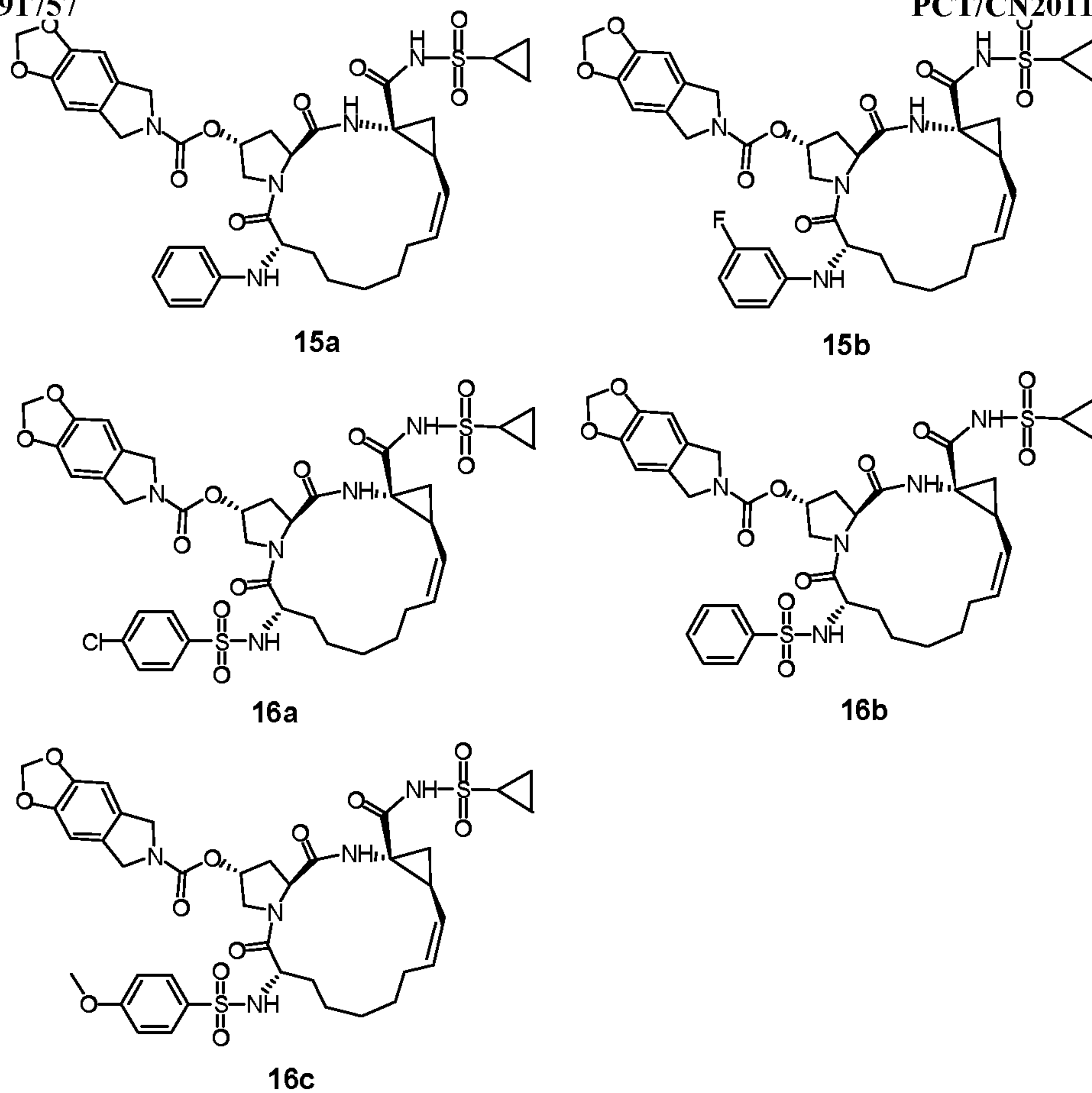
Figure 6: Structure of Compounds 15a-15b , 16a-16c
