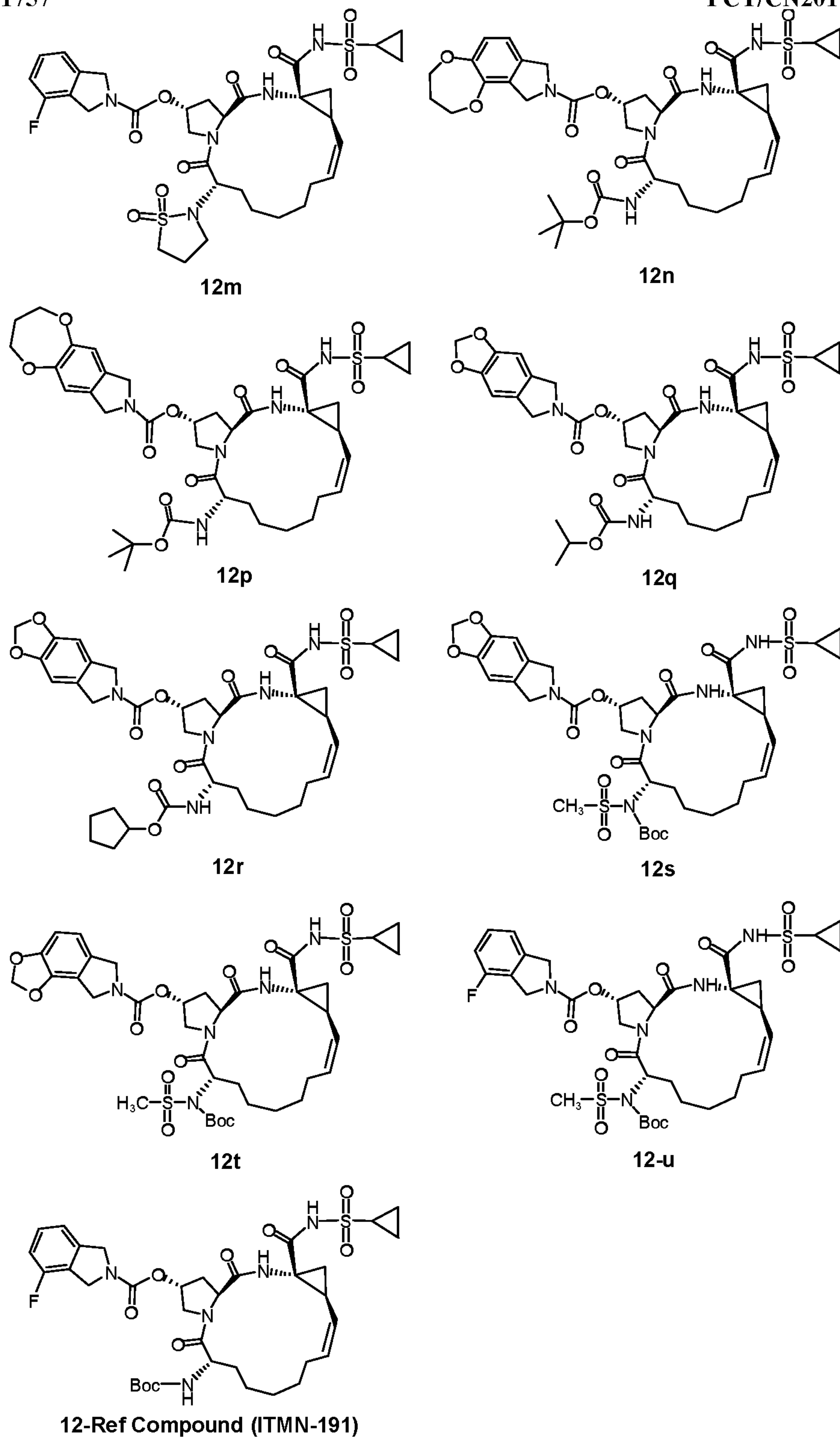
Figure 5: Structure of Compounds 12a-12u and 12-Ref
