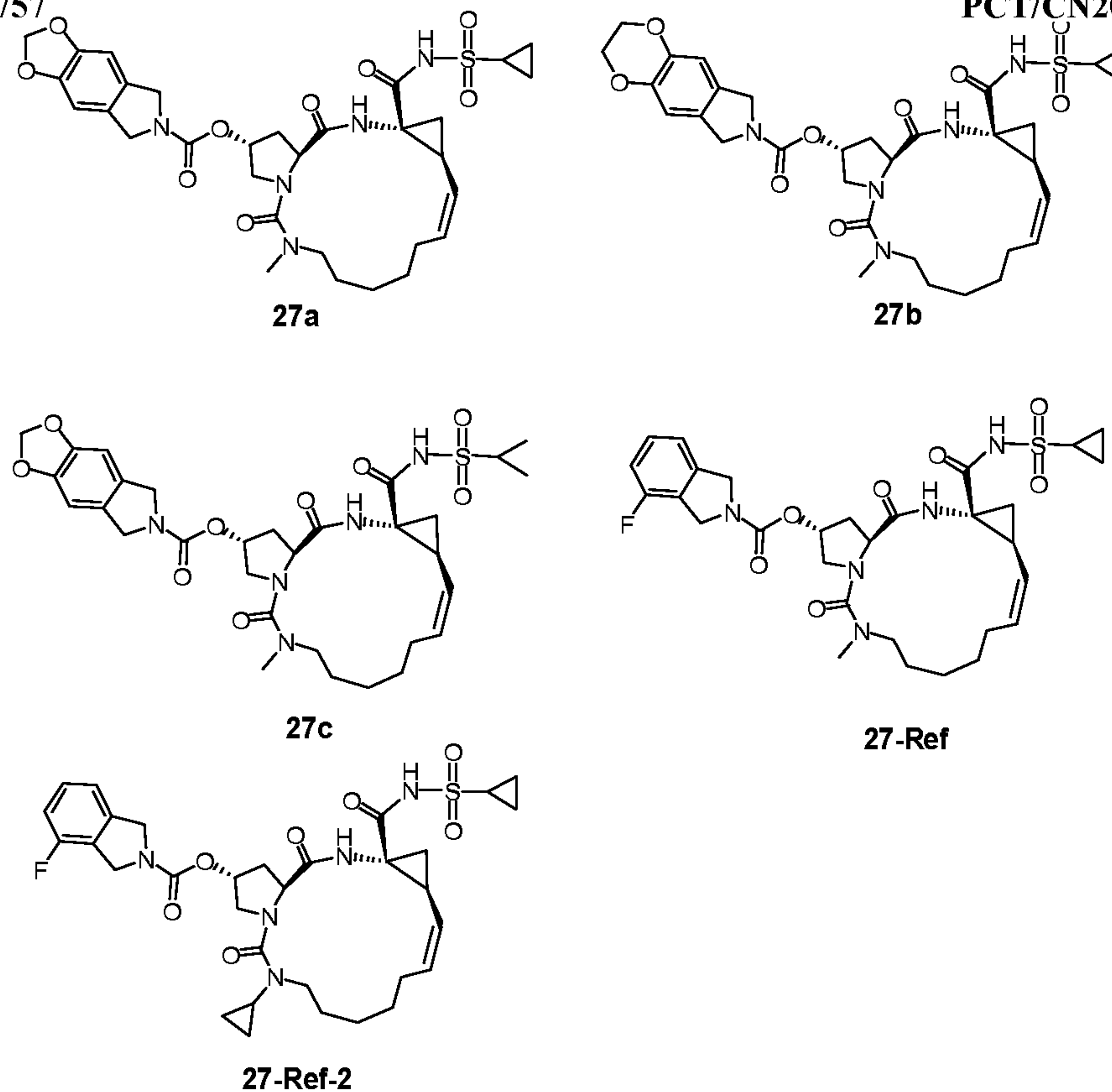
Figure 8: Structure of Compounds 27a-27c and 27-Ref
