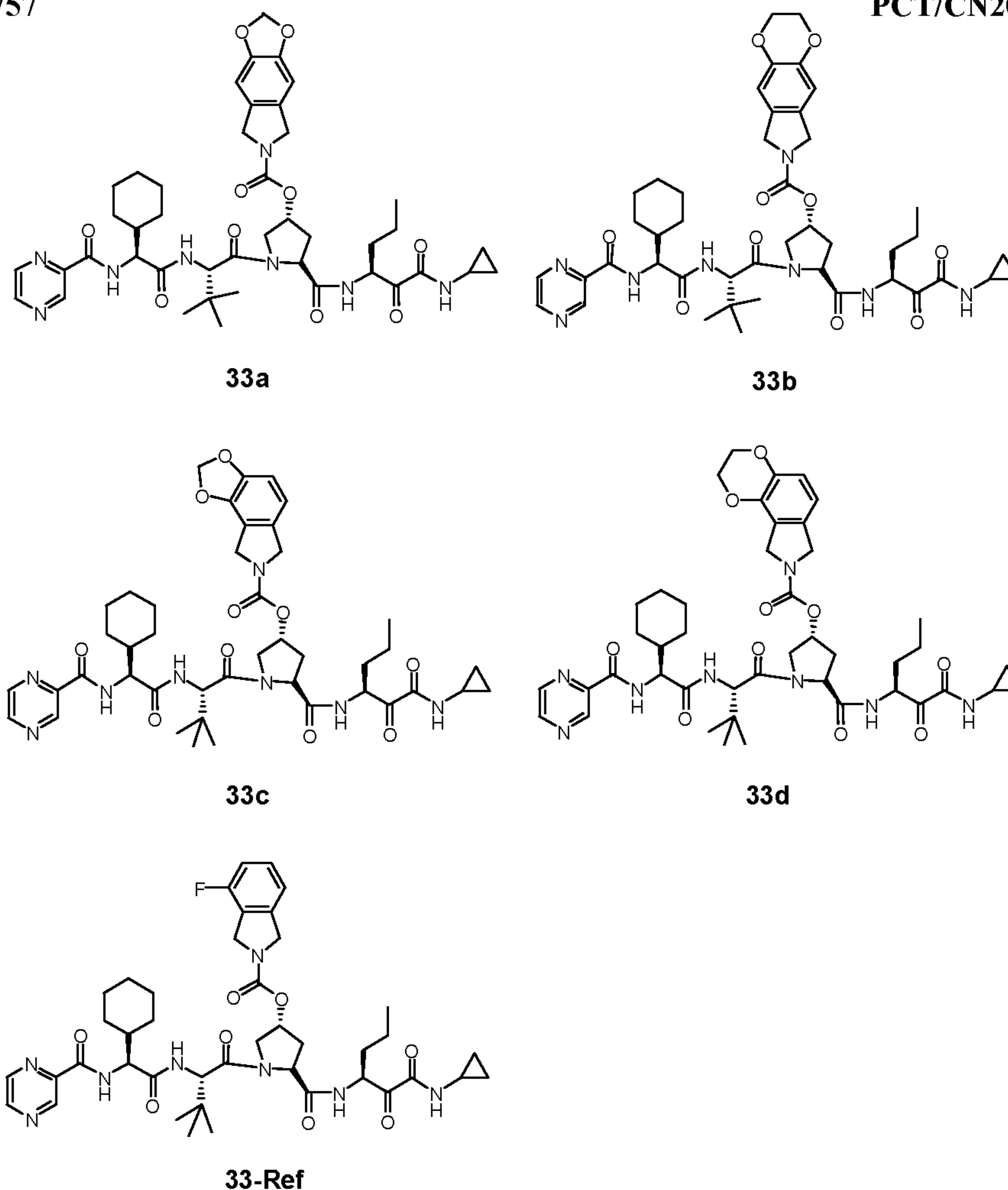
Figure 11: Structure of Compounds 33a-33d and 33-Ref
