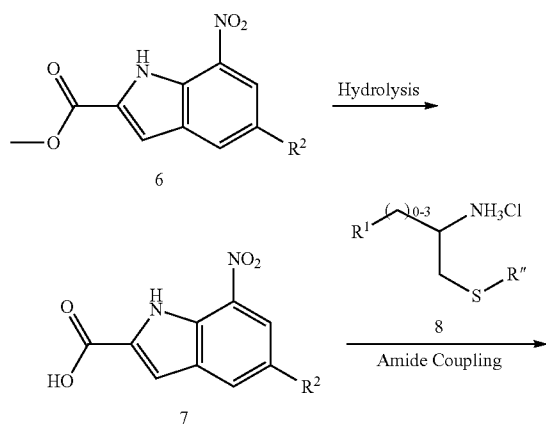
Reaction Scheme 3
