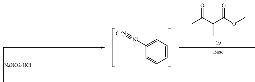
Reaction Scheme 5
