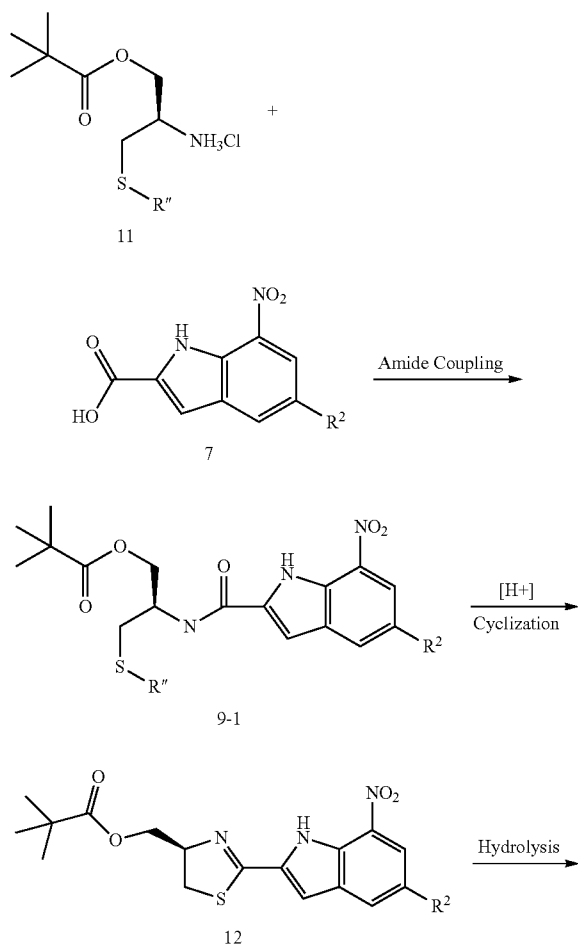
Reaction Scheme 4
