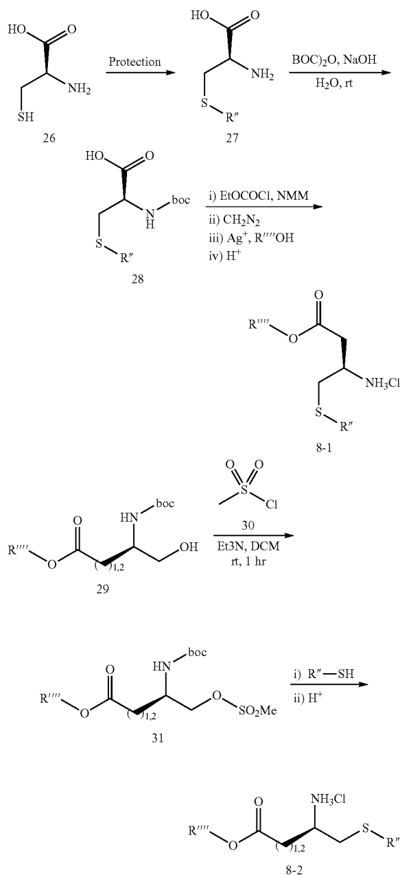
Reaction Scheme 8
