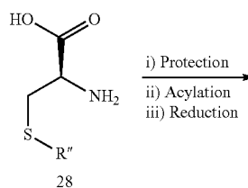
Reaction Scheme 9
