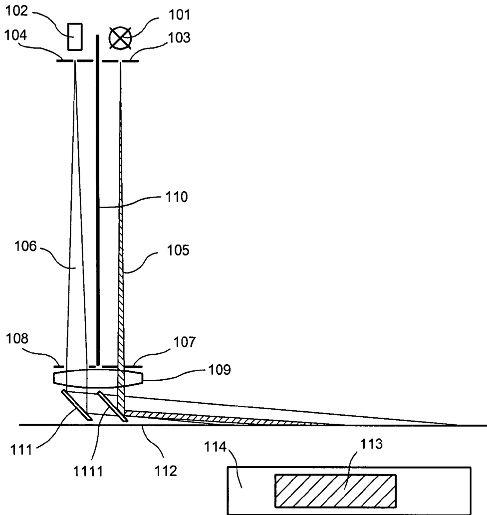
Fig. 1 PRIOR ART
