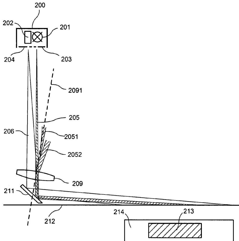
Fig. 2 PRIOR ART
