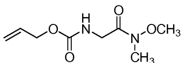
44 allyl 2-(methoxy(methyl)- amino)-2-oxoethylcarbamate
