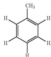
toluene
