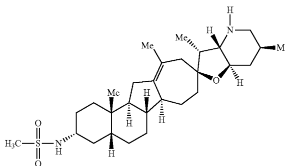
IPI-926
