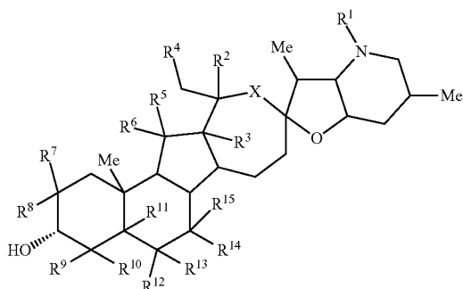
(R)-(II)
