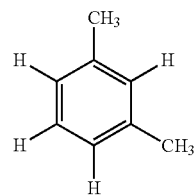
m-xylene
