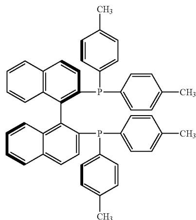
(R)-Tol-BINAP
