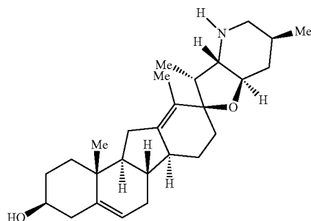
cyclopamine
