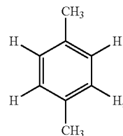
p-xylene
