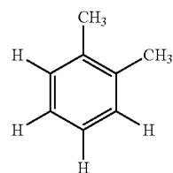
o-xylene
