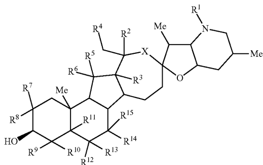
(S)-(II)
