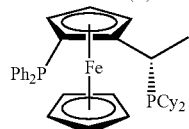
(R,S)-JOSIPHOS
