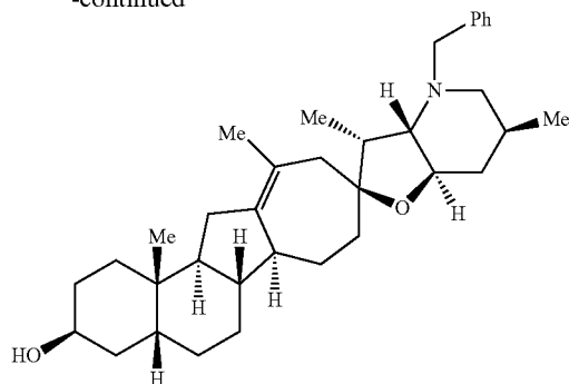
(S)-(II-a)
