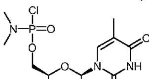
Compound (E1)
