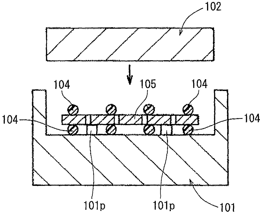
FIG. 9 PRIOR ART
