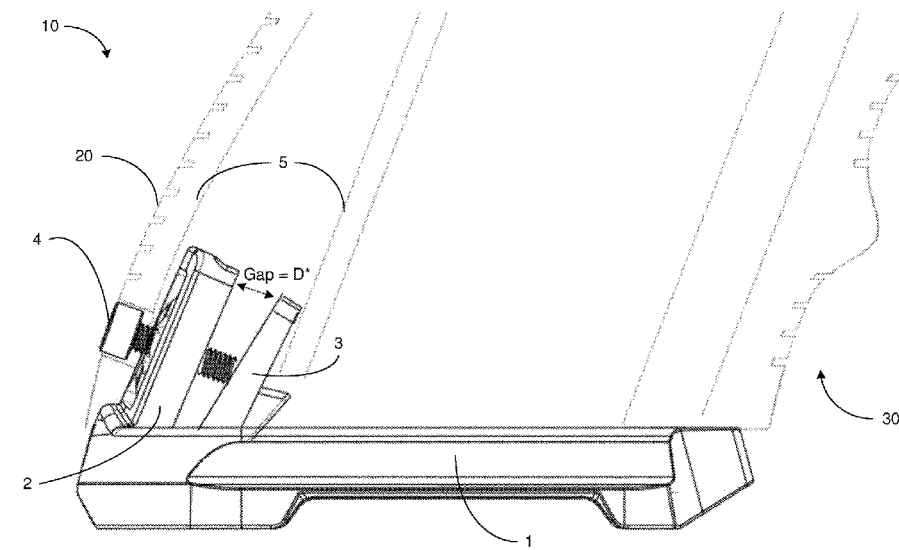
Continue to screw in screw 4 until gap between first tab 2 and second tab 3 is sufficiently expanded to firmly hold magazine funnel 1 in place
