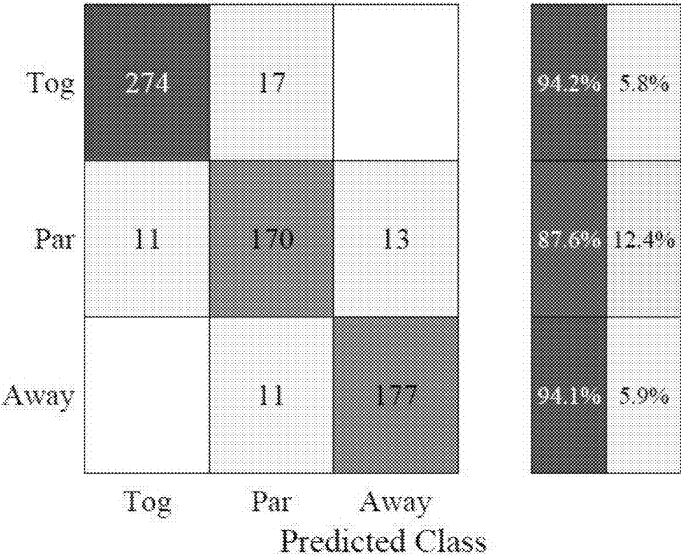
Direction Confusion Matrix
