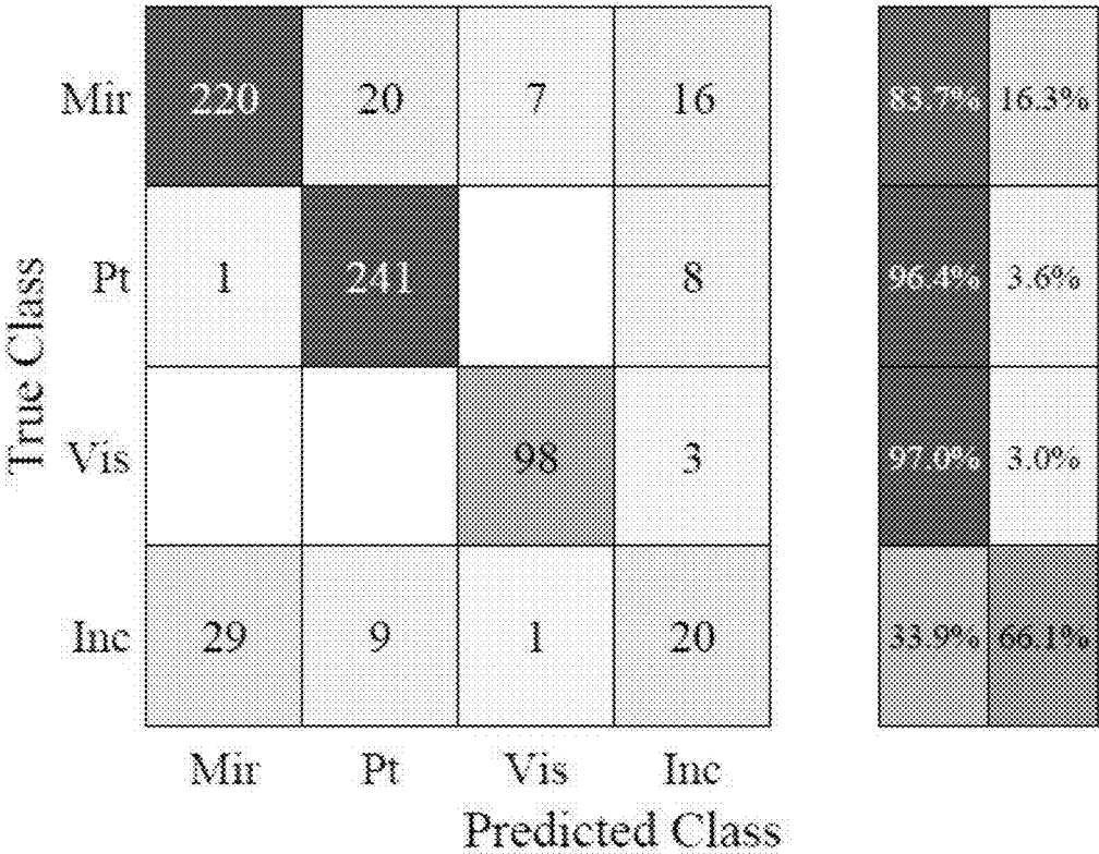
Symmetry Confusion Matrix
