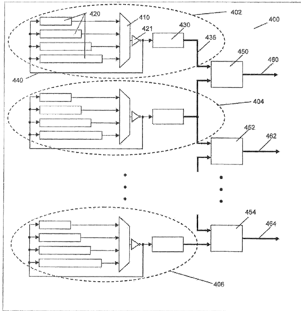
Figure 11, Asymmetric Unclonable Function Structure
