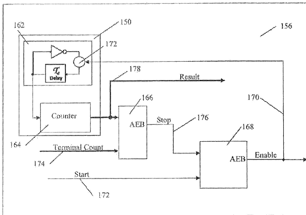
Figure 9, Reference Cell
