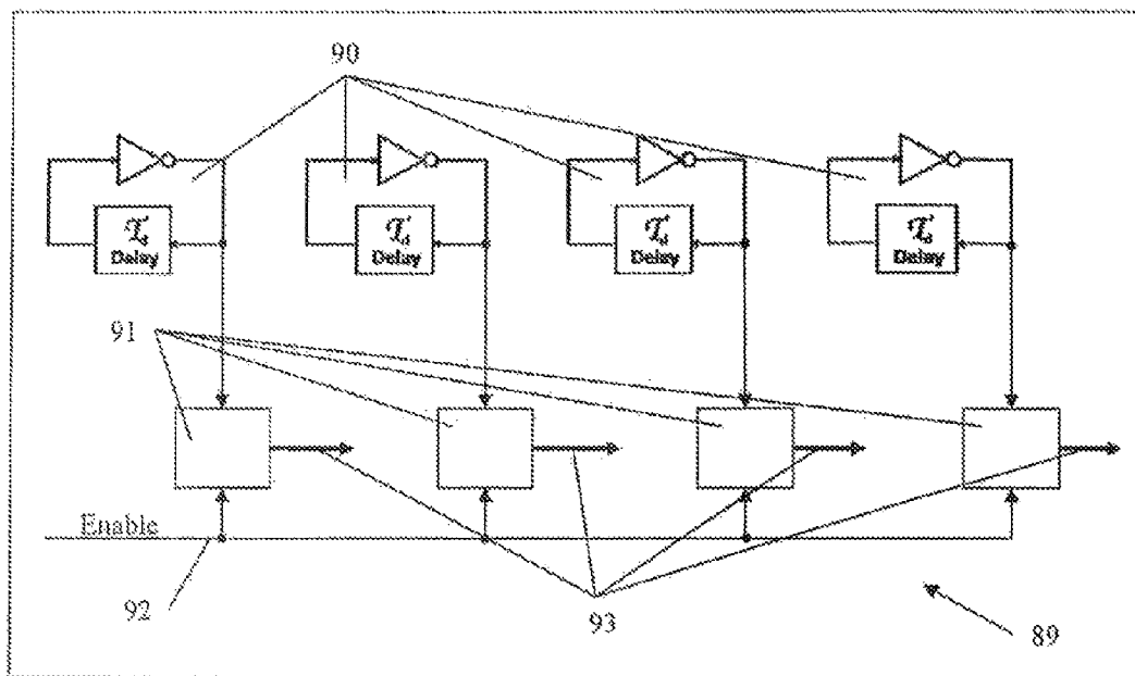
Figure 6, Ring Oscillator Array
