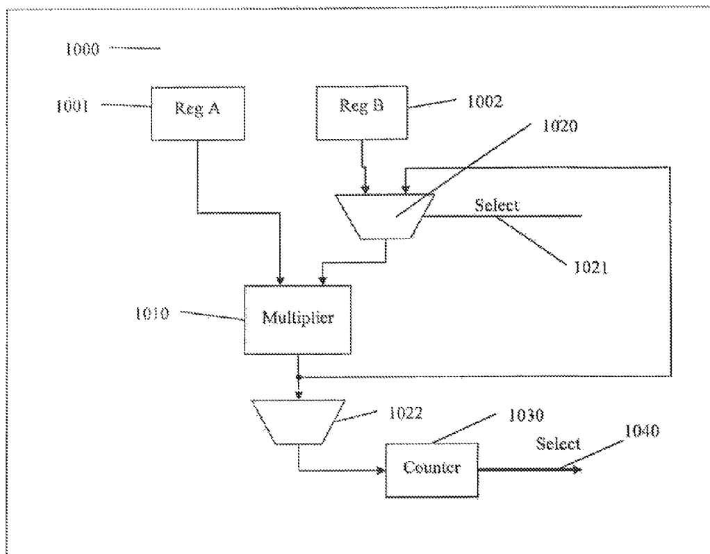
Figure 15, Multiplier Based AUF Cell
