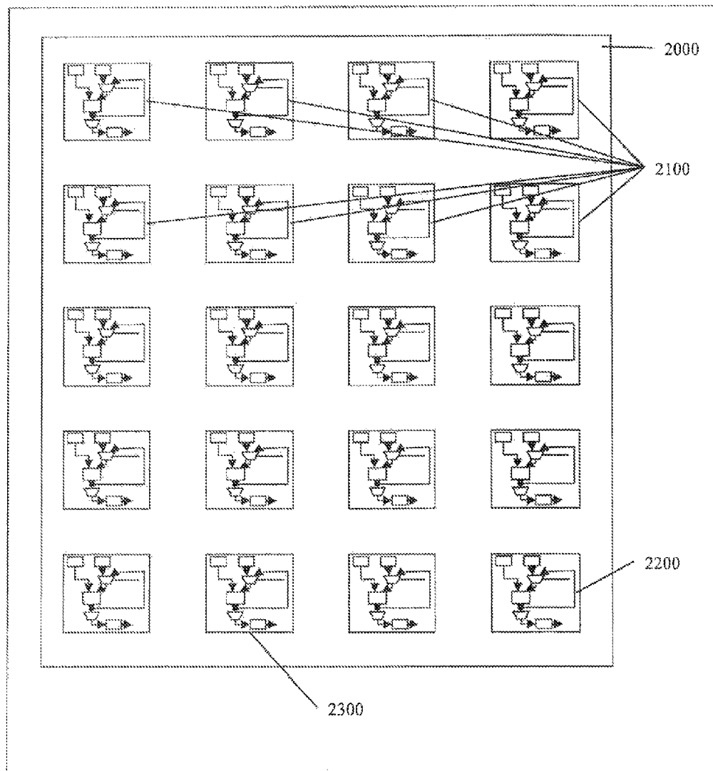
Figure 16, Asymmetric Unclonable Array Constructed of Multiplier-Based Cells/Elements
