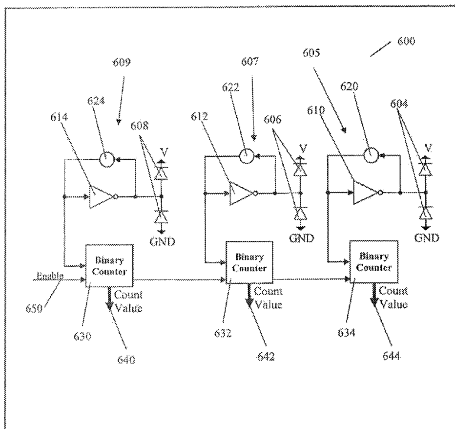
Figure 14, Diode Incorporated AUF cells
