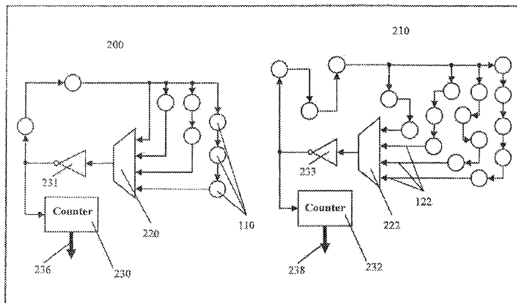
Figure 10, Asymmetric Ring Oscillators with Multiplexed route Lengths
