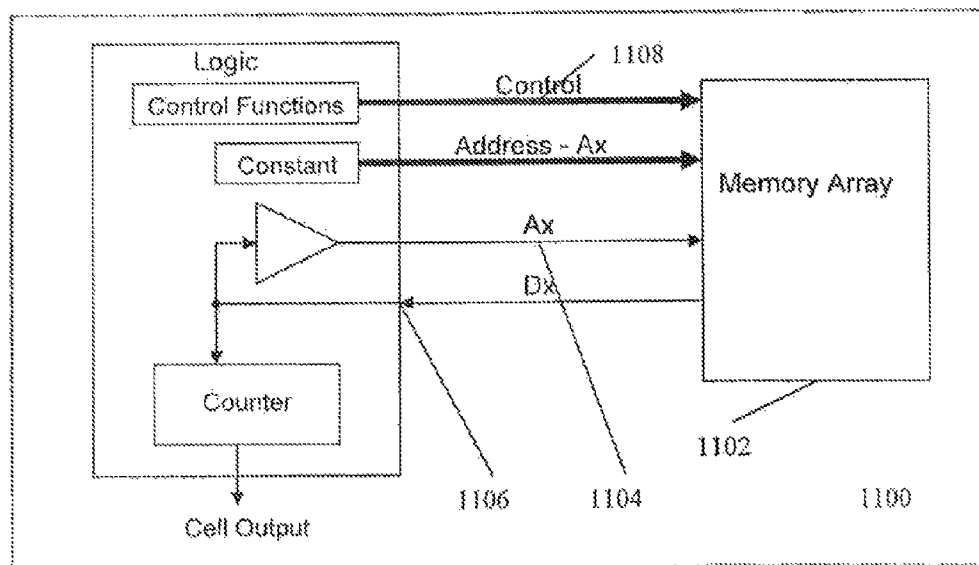
Figure 17, Memory Based AUF Cell
