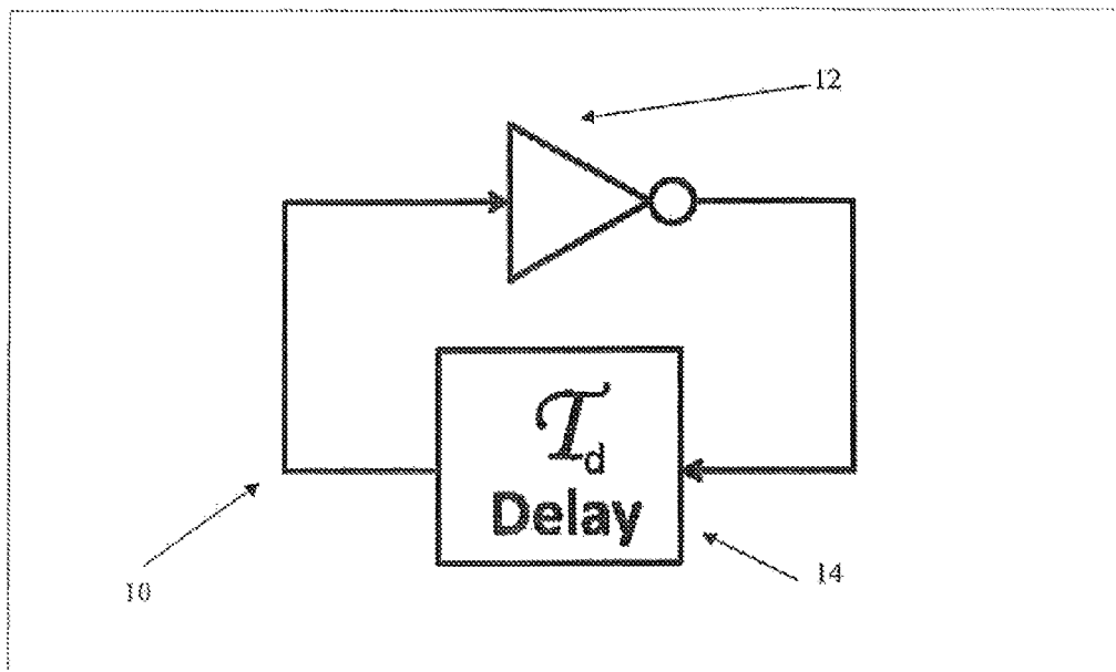
Figure 5. Basic Oscillator
