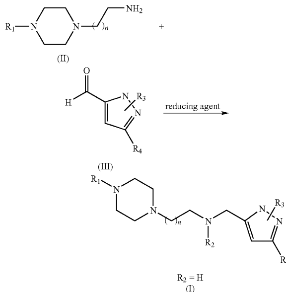
Reaction Scheme 1
