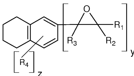
Structure III
