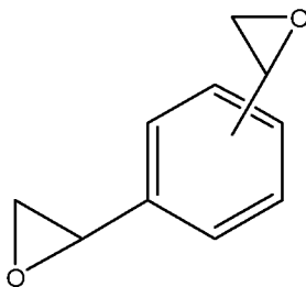
Structure V
