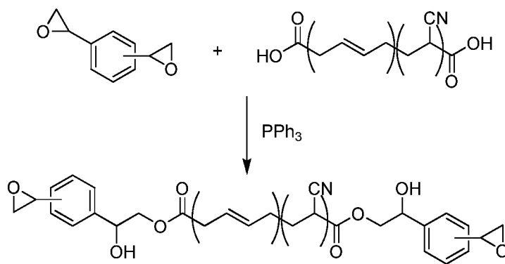
Scheme I
