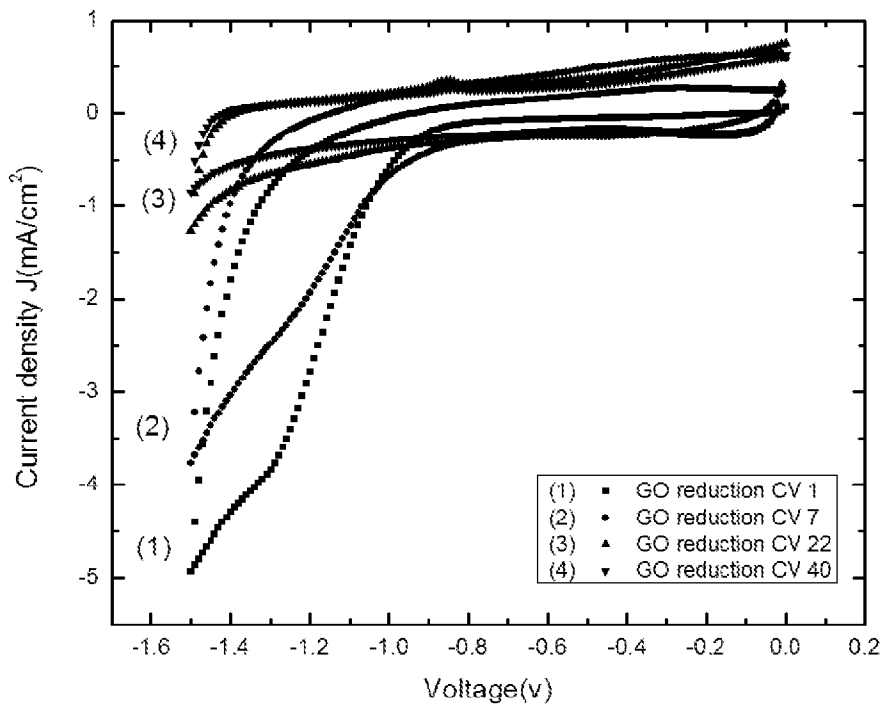
Figure 10. Cyclic voltammograms taken at 1 st , 7 th , 22 nd and 40 th cycle of ERGO/GCE
