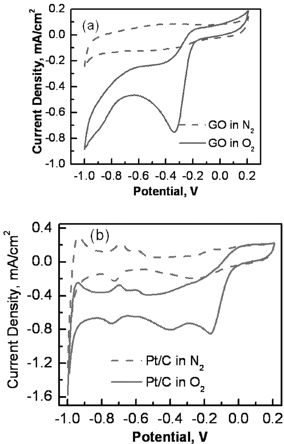
Figure 6(a). Comparison of cyclic voltammetric response of GO in N 2 and O 2 saturated solution. (b) Comparison of Pt/C response in N 2 and O 2 saturated solution
