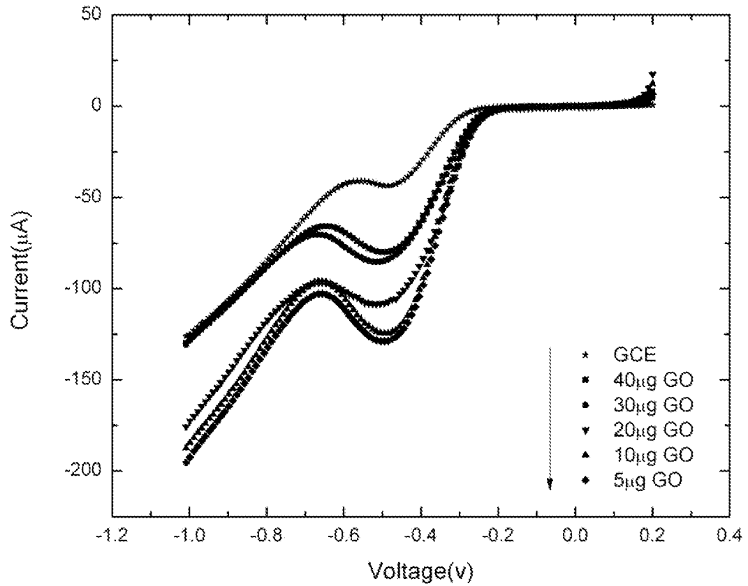
Figure 13. Linear-sweep voltammetry curves of bare GCE electrode compared with various GO mass (in O_2 ).
