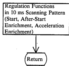
Flowchart No. 3:
