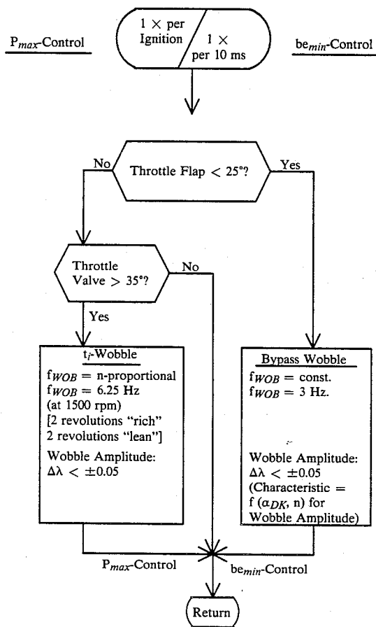
Flowchart No. 4: Test Signal Generator
