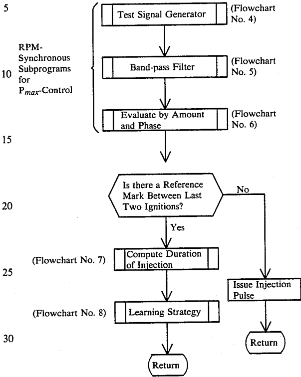
Flowchart No. 3:
