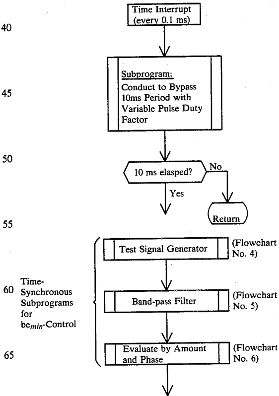
Flowchart No. 3:
