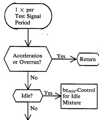
Flowchart No. 6: Evaluate by Amount and Phase
