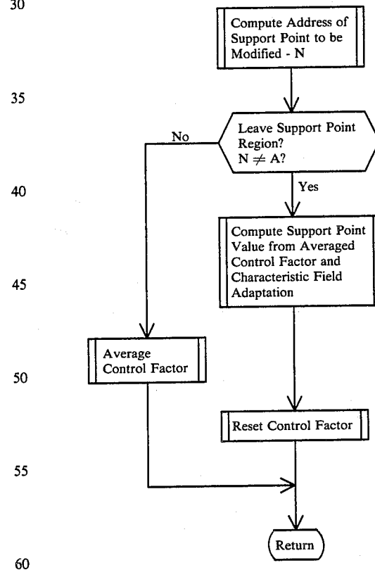
Flowchart No. 8: Characteristic Field Learning Strategy
