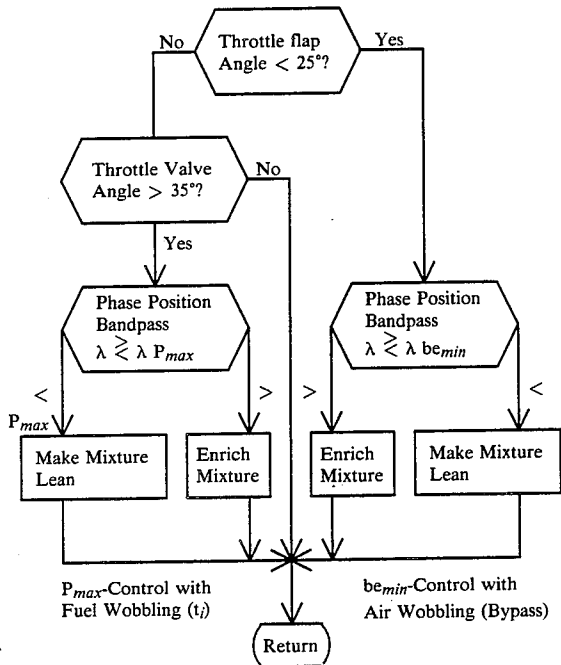
Flowchart No. 6: Evaluate by Amount and Phase
