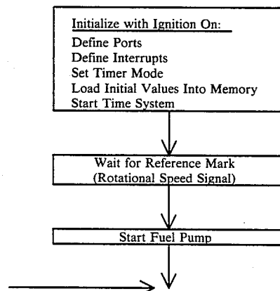
Flowchart No. 1: Main Program
