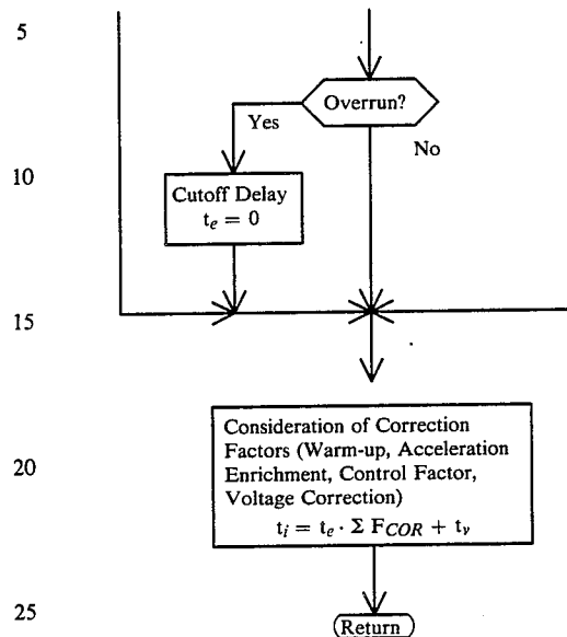
Flowchart No. 7: Compute Duration of Injection
