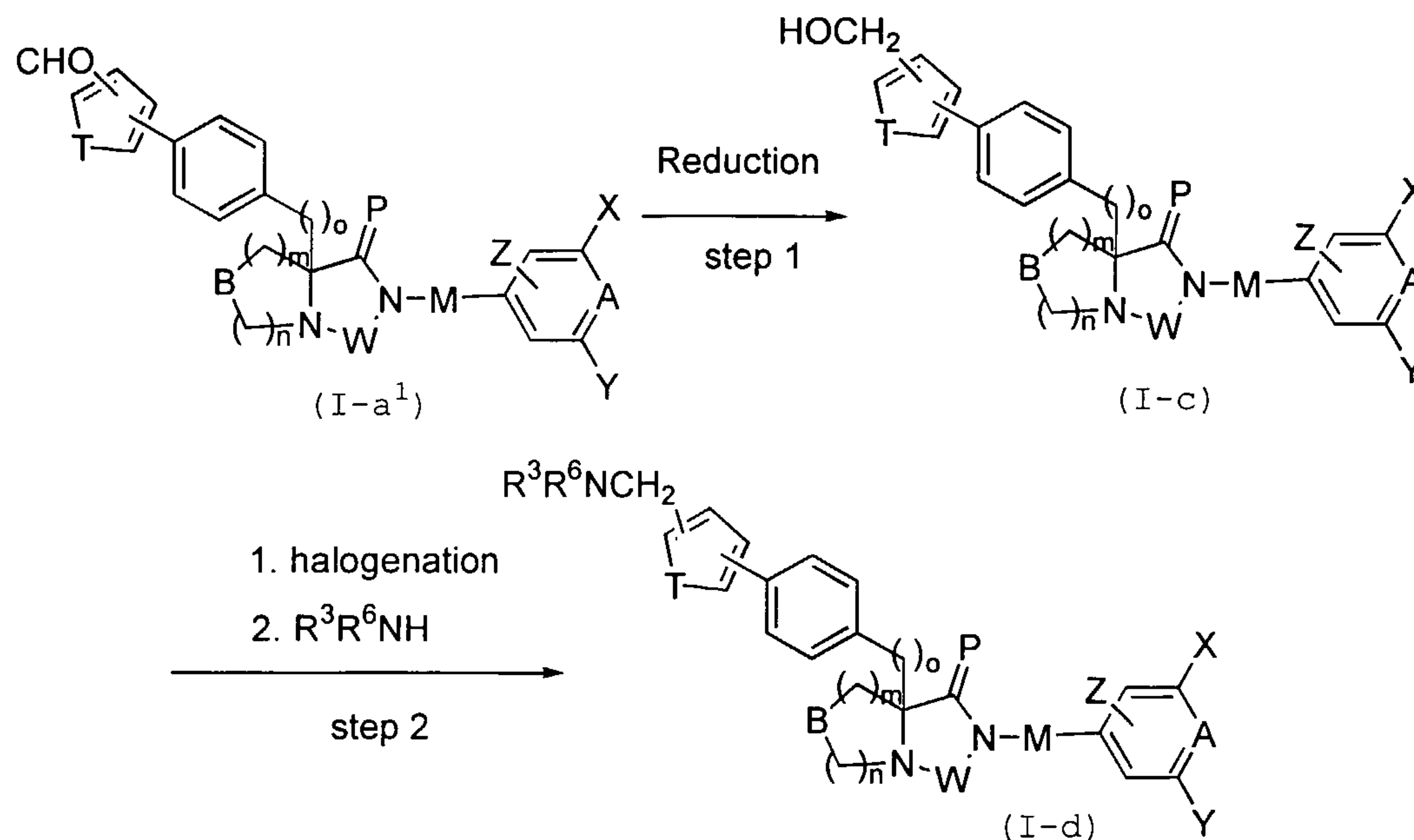
Scheme 2.
