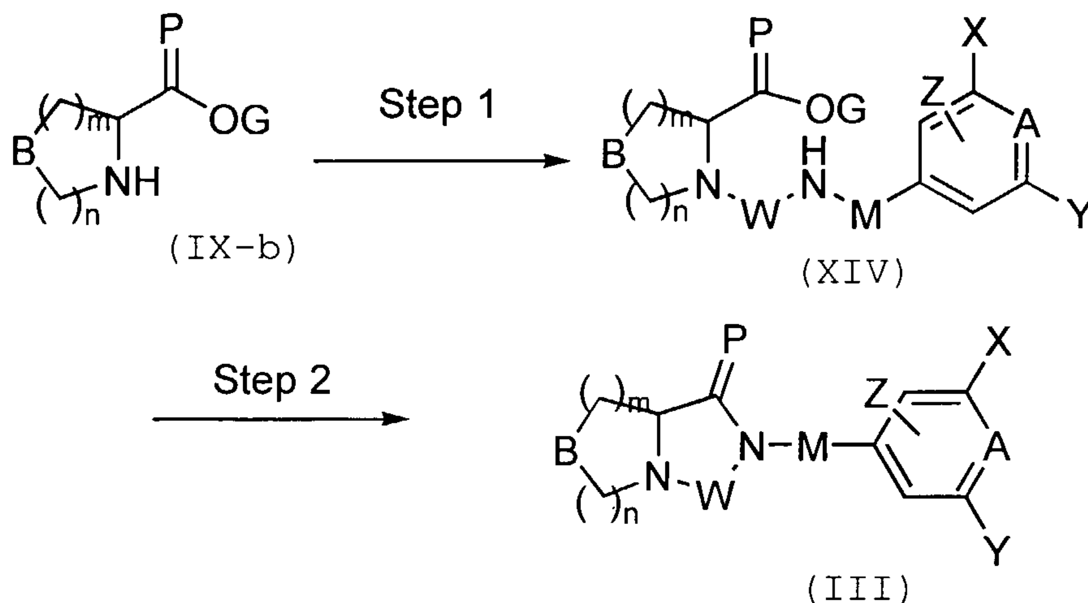
Scheme 9.
