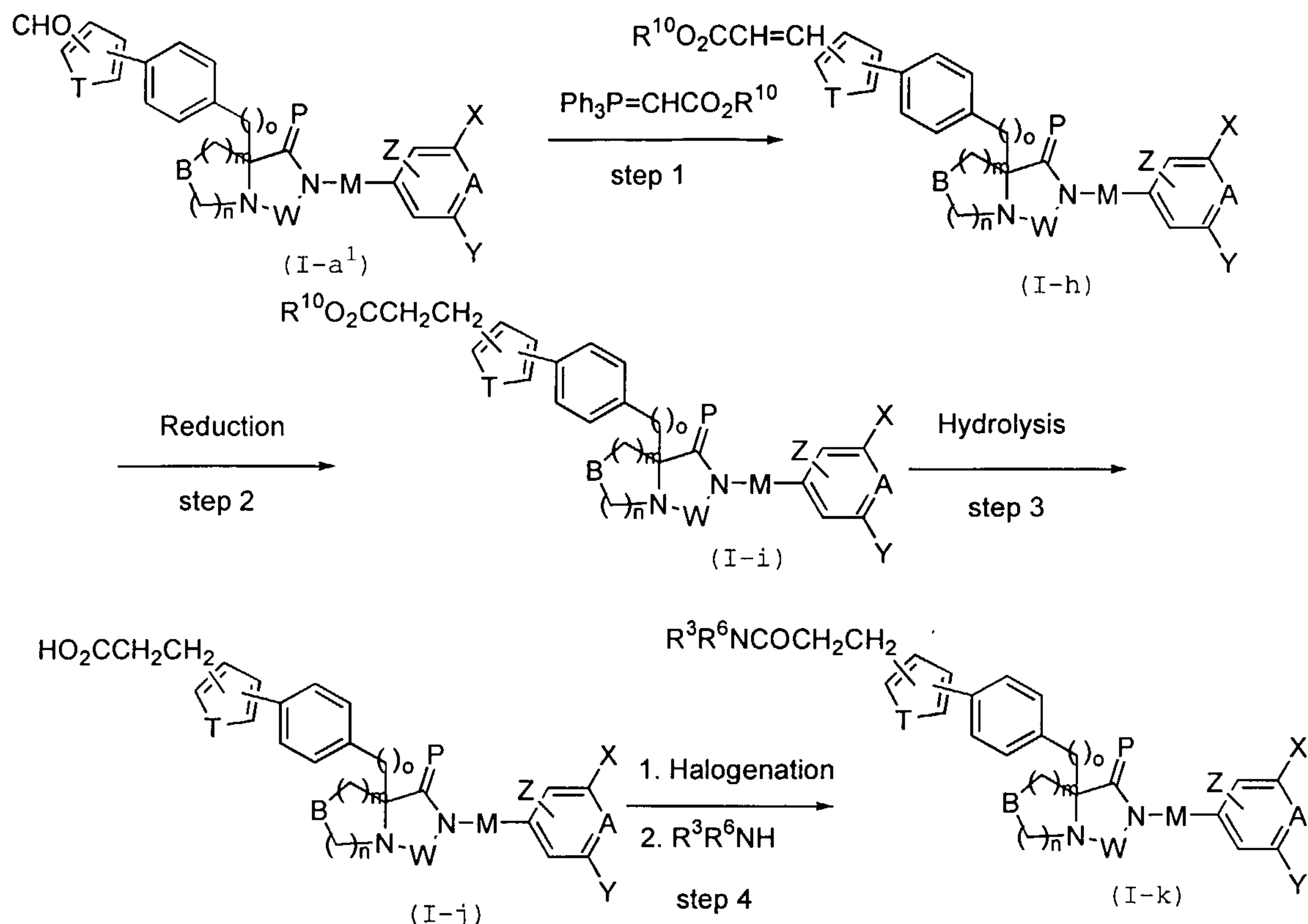
Scheme 4.
