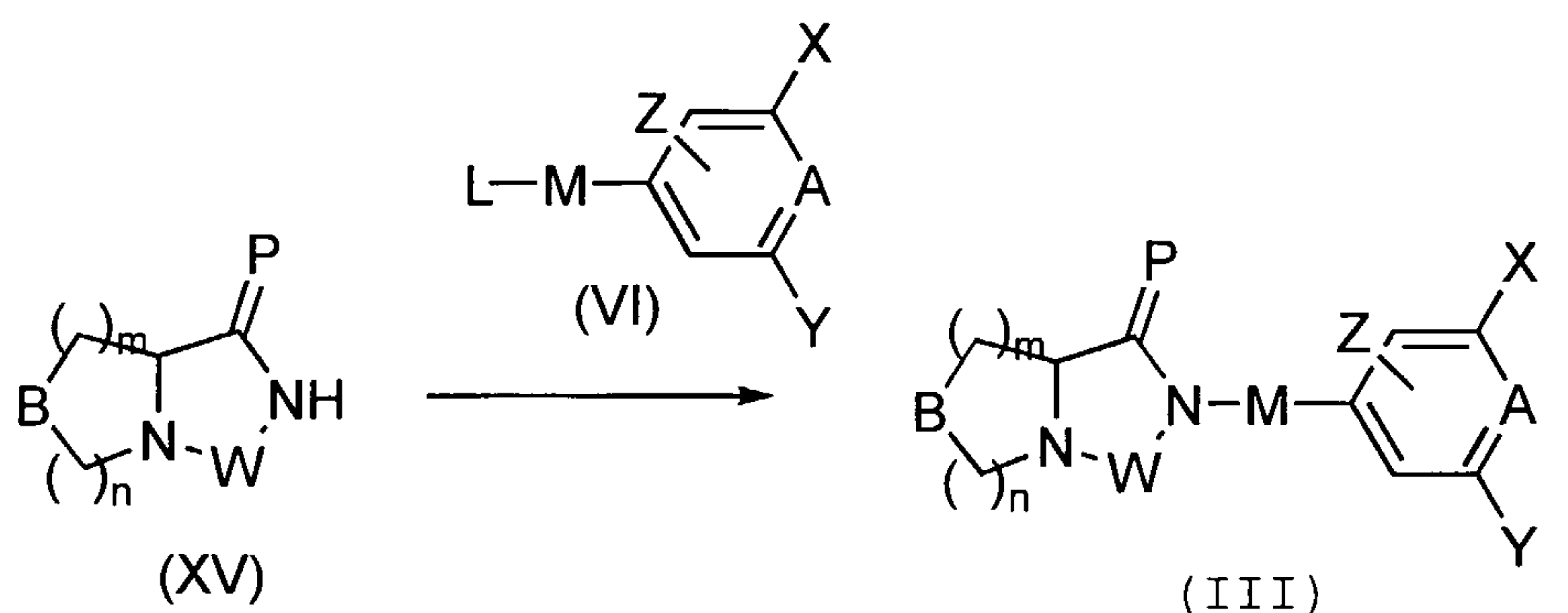
Scheme 10.
