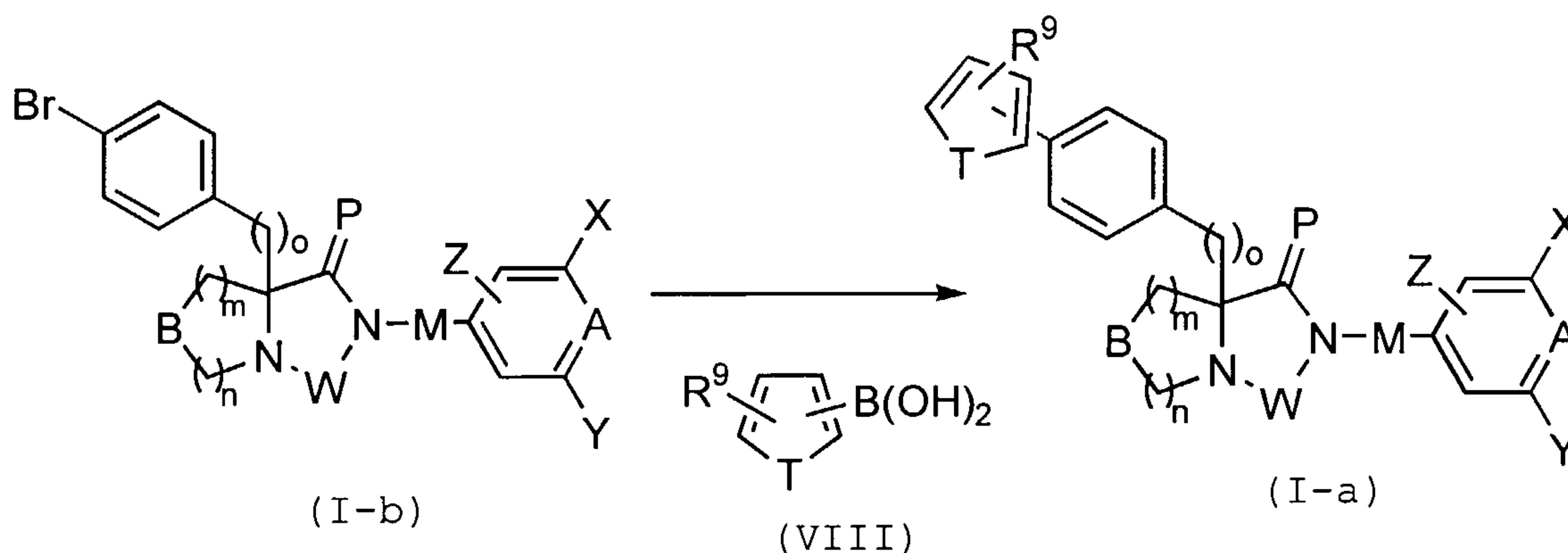
Scheme 1.
