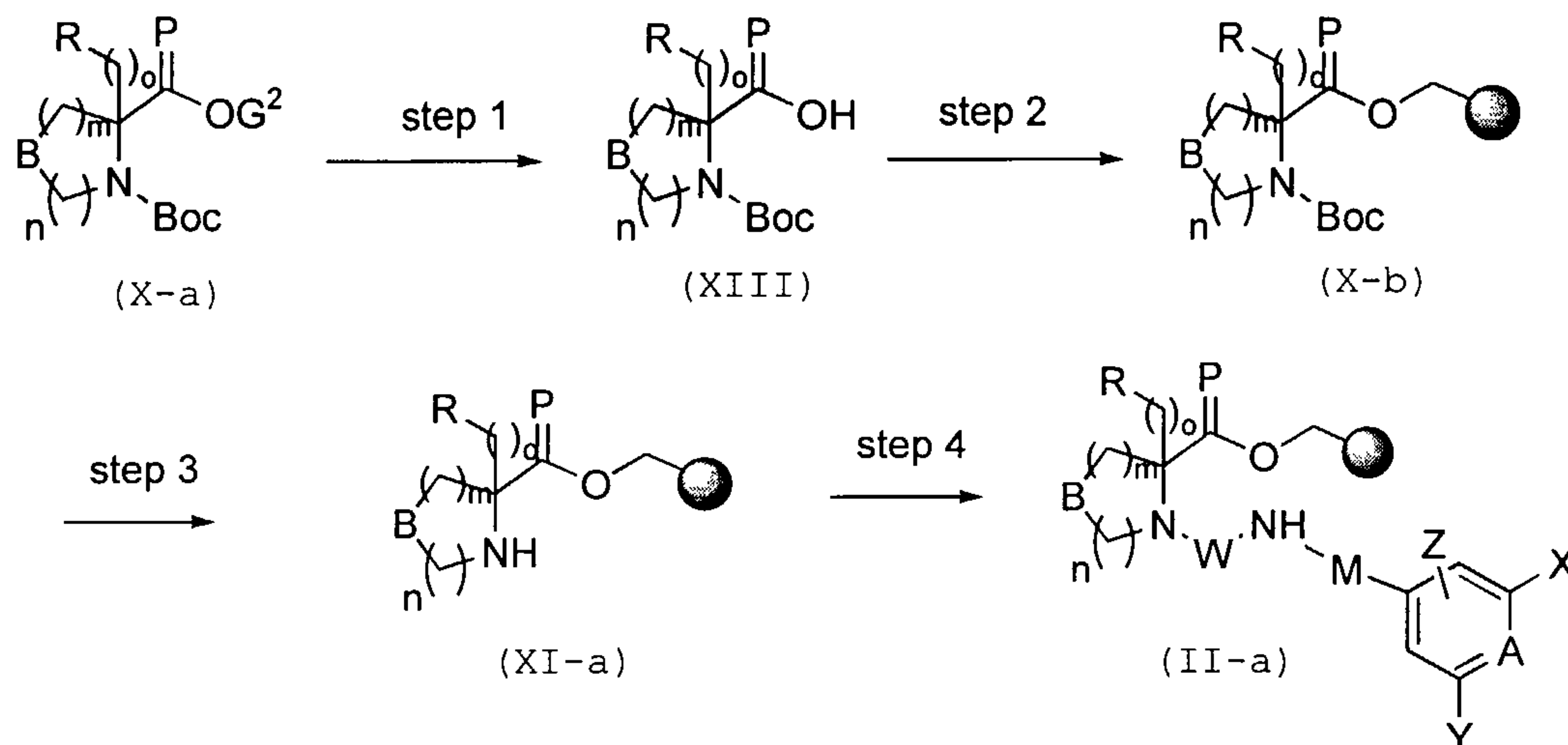
Scheme 8.
