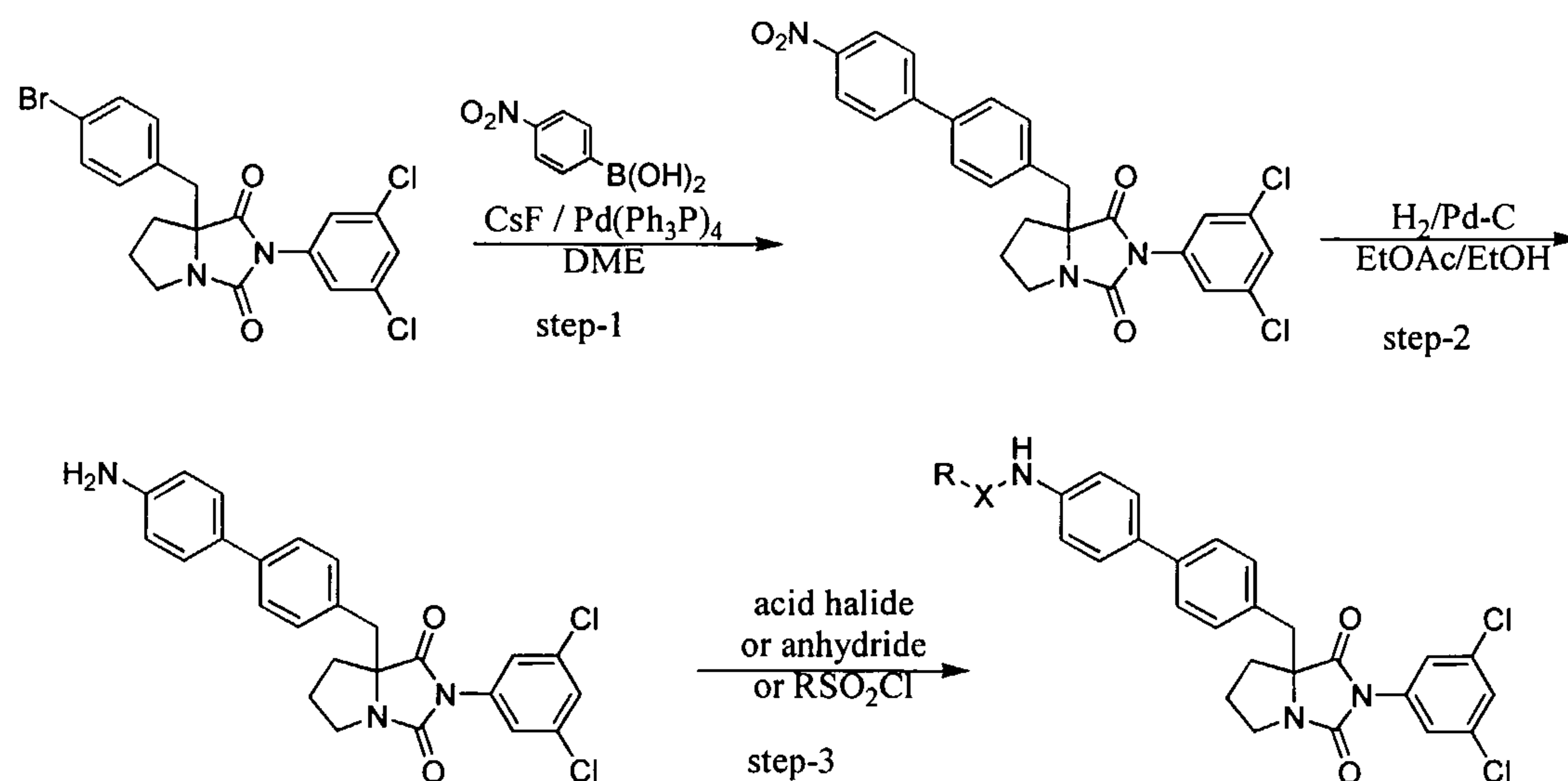
Scheme 12:
