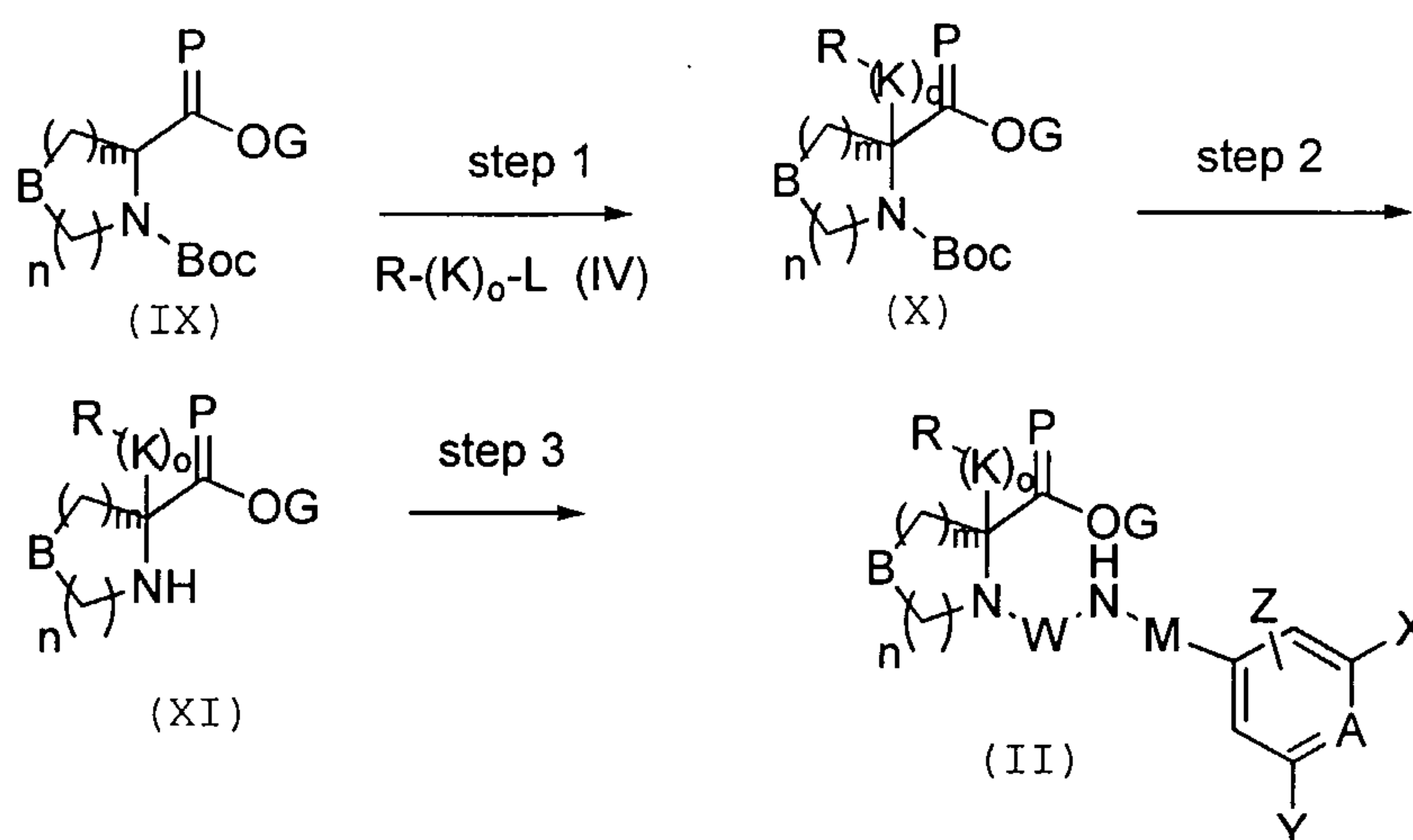
10 Scheme 7.
