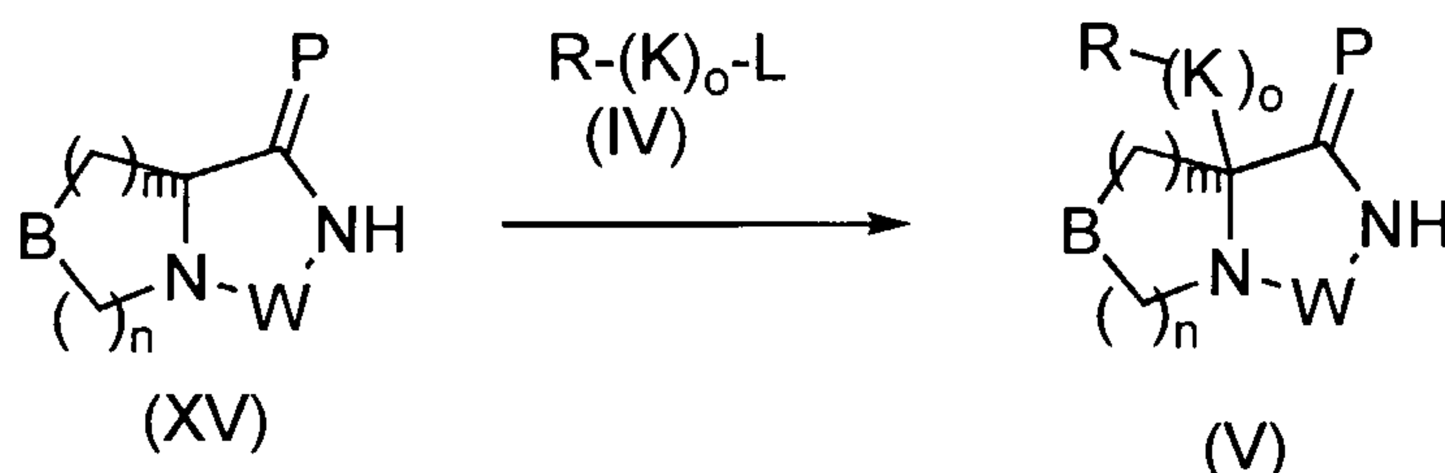
Scheme 11.
