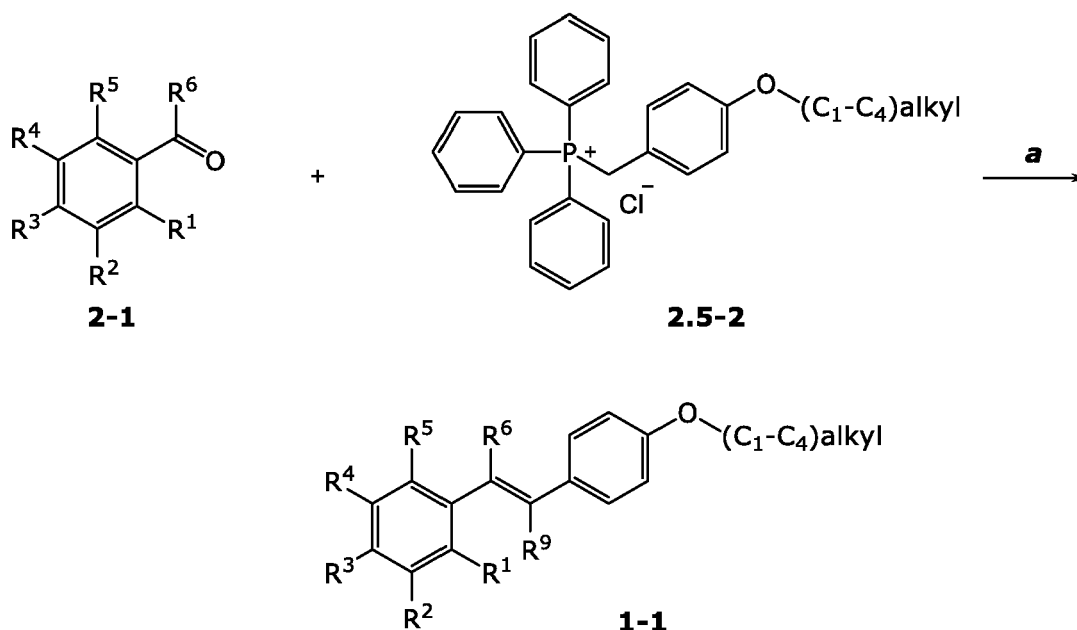
Scheme 2.5
