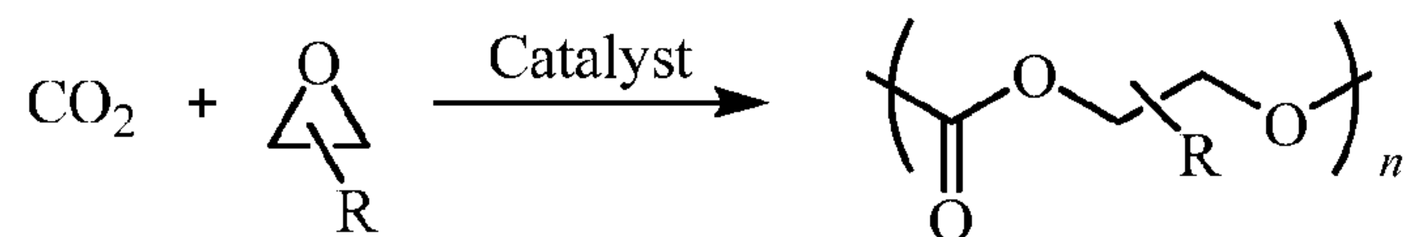
SCHEME 1
