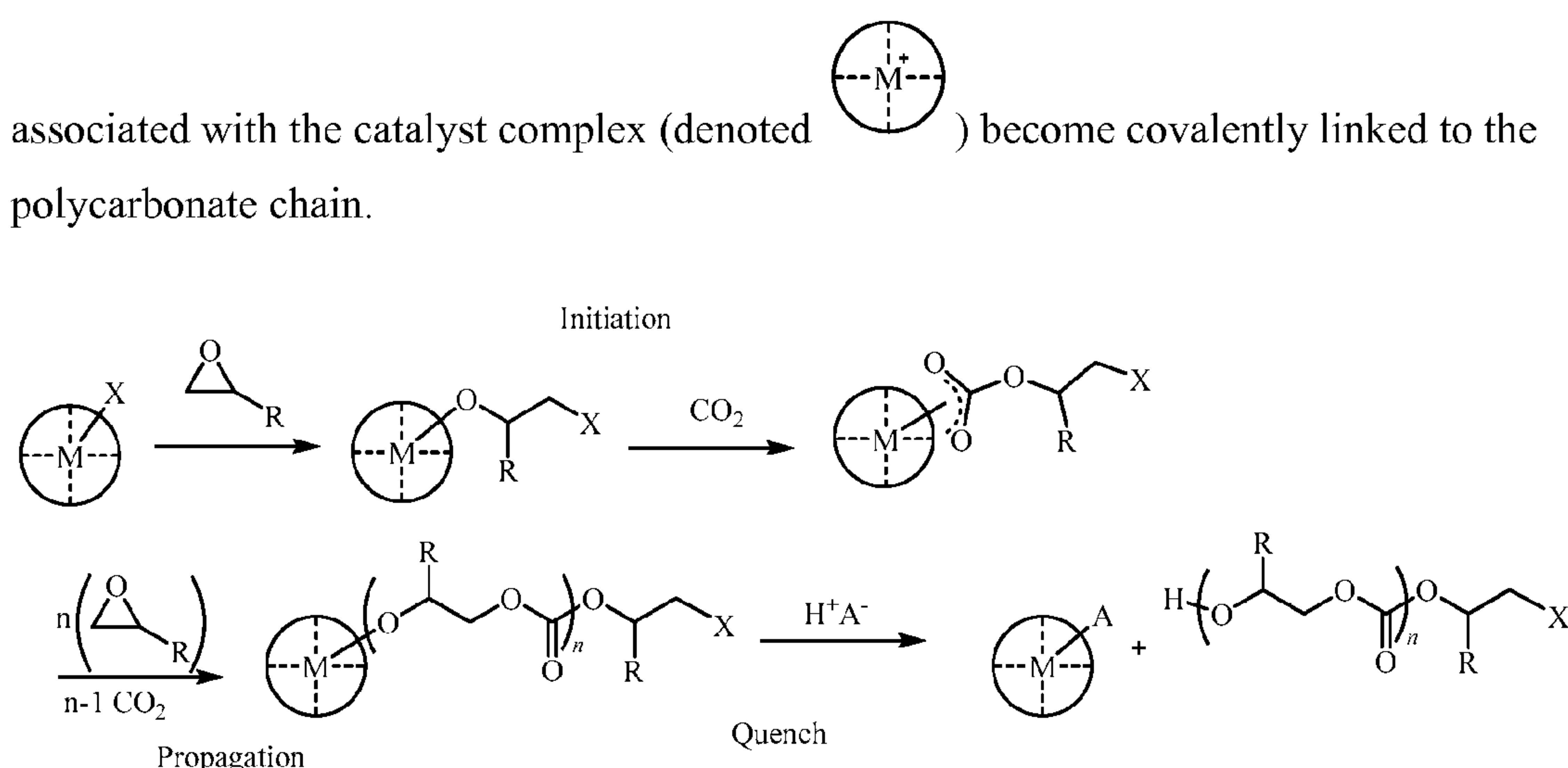
SCHEME 2
