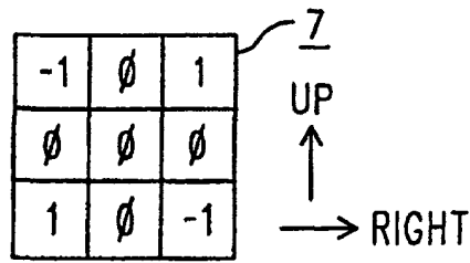
THE "STANDARD" FILTER
