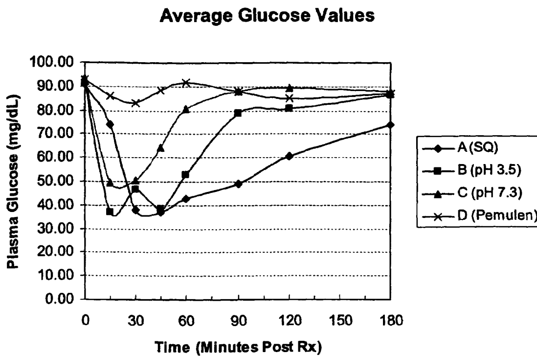
Figure 1. Average Glucose Values (n = 8)
