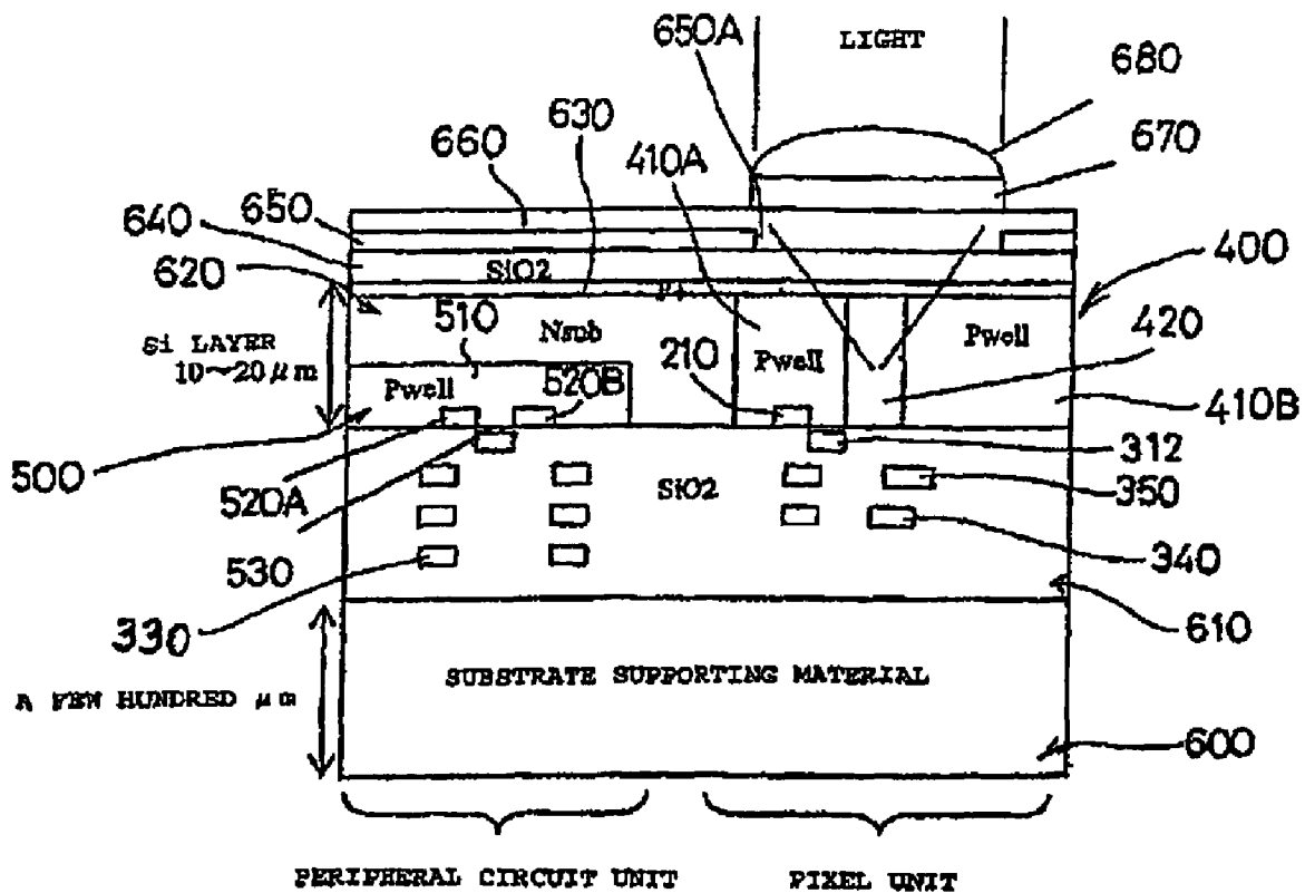
FIG. 12 (PRIOR ART)
