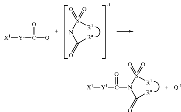
Reaction Scheme A'
