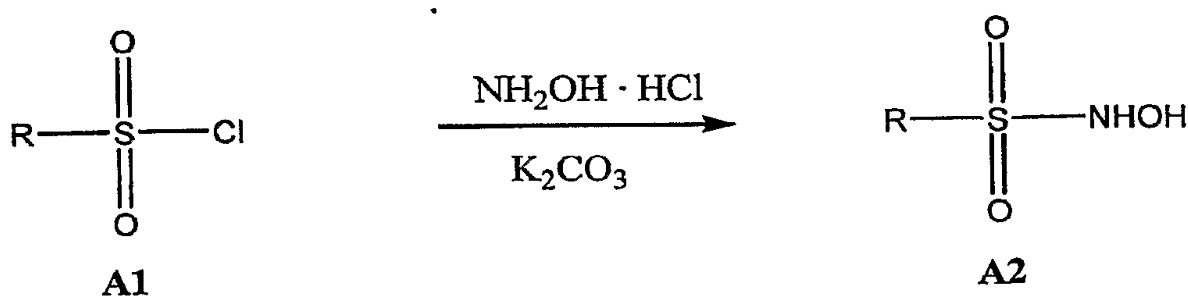
Scheme A. General Synthesis of N -Hydroxysulfonamides.
