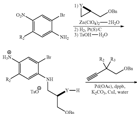
Scheme 4: Coupling of the Acid Chloride and Amine Moiety
