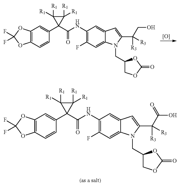
Scheme 8: One Pot Oxidation to Carboxylic Acid
