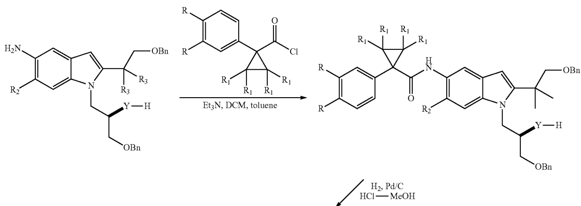
Scheme 4: Coupling of the Acid Chloride and Amine Moiety
