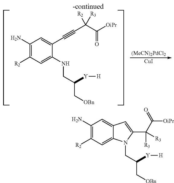
Scheme 11: Hydrolysis of Isopropyl Ester
