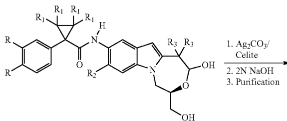
Scheme 6: Oxidation and Hydrolysis to Produce Compounds of Formula I
