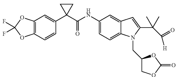
Scheme 1: Synthesis of the Acid Chloride Moiety
