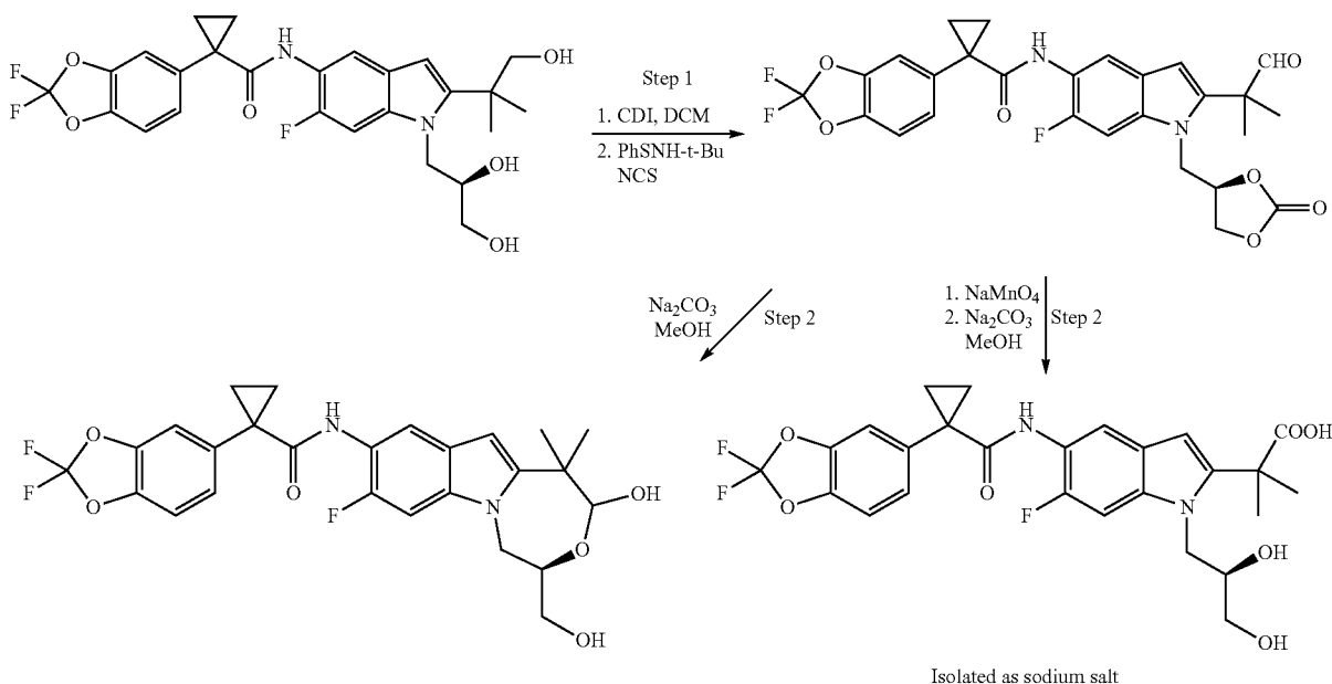
Scheme 12: Synthesis of Compounds of formula Ia and IIa where R 2 is F
