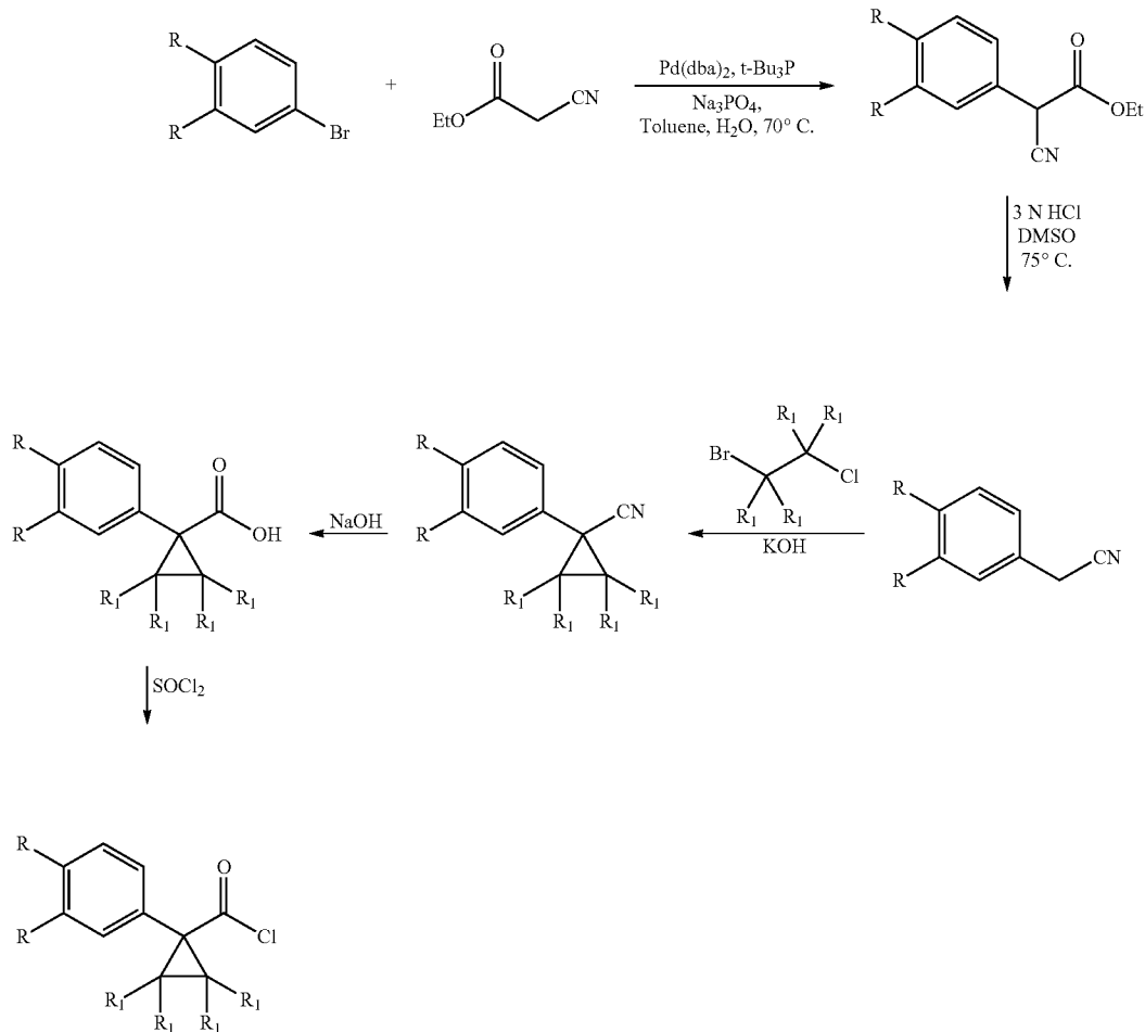
Scheme 2: Alternative Synthesis of the Acid Chloride Moiety
