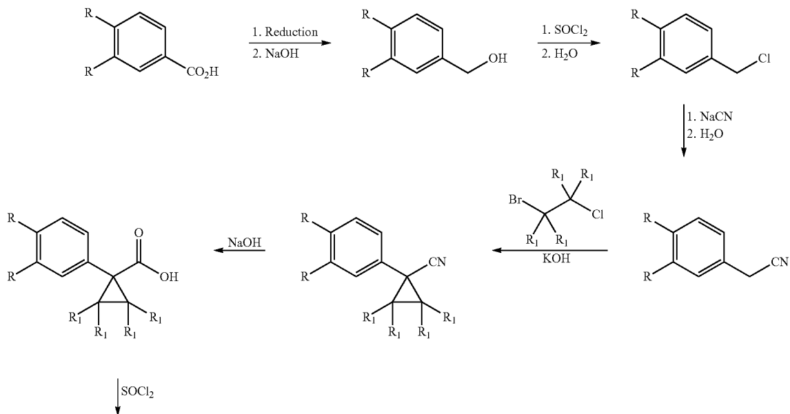
Scheme 1: Synthesis of the Acid Chloride Moiety
