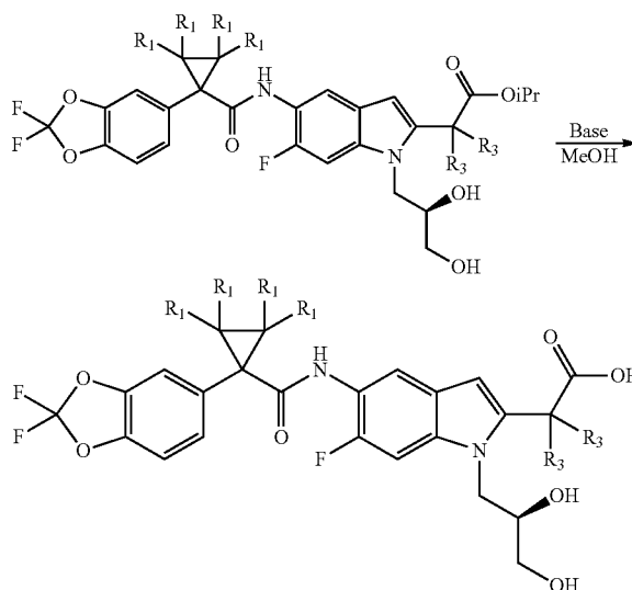
Scheme 11: Hydrolysis of Isopropyl Ester
