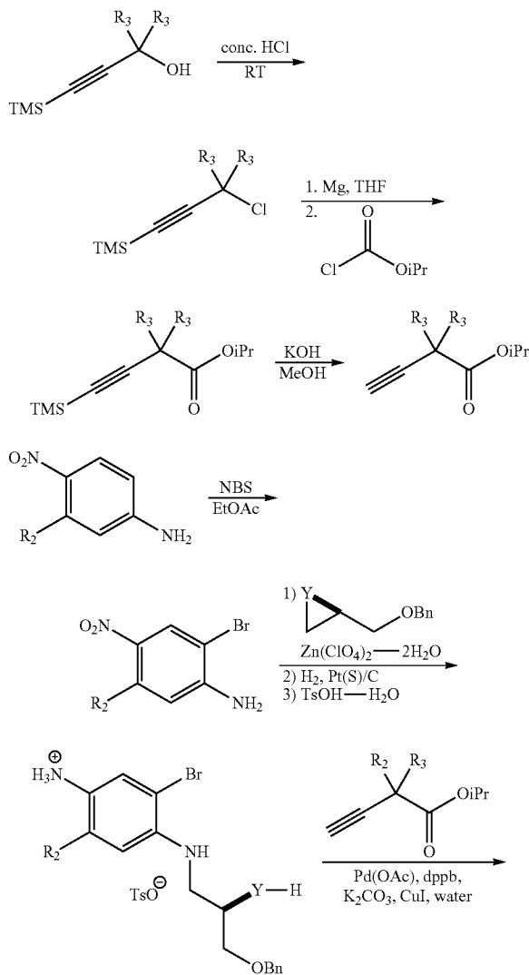
Scheme 10: Alternative Synthesis of Compound of Formula I
