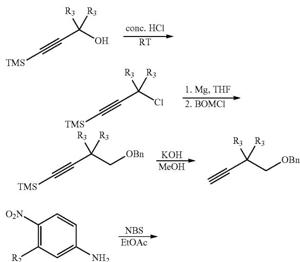
Scheme 3: Synthesis of the Amine Moiety
