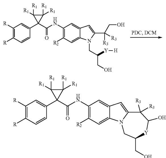
Scheme 5: Ring Closure to Produce Compounds of Formula II
