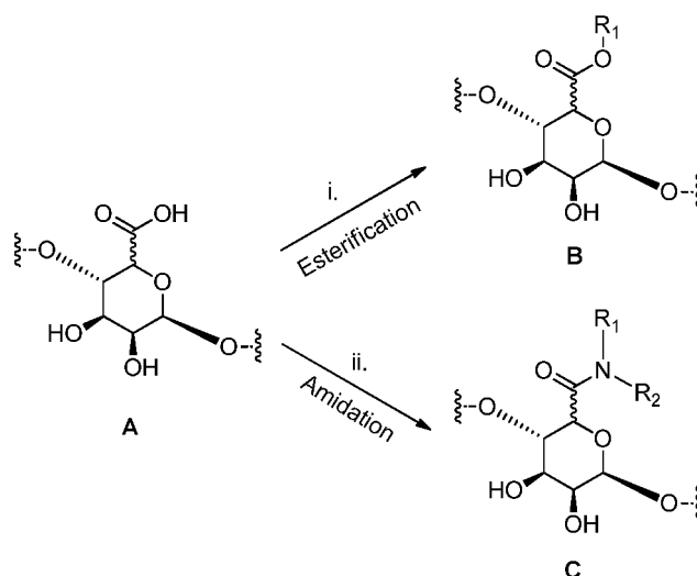
Scheme 1. Representative Reaction Conditions: i. HO-R 1 , 2-Chloro-4,6-dimethoxy-1,3,5-triazine (CDMT), N-methyl morpholine (NMM); ii. HNR 1 R 2 , CDMT, NMM (reference only).
