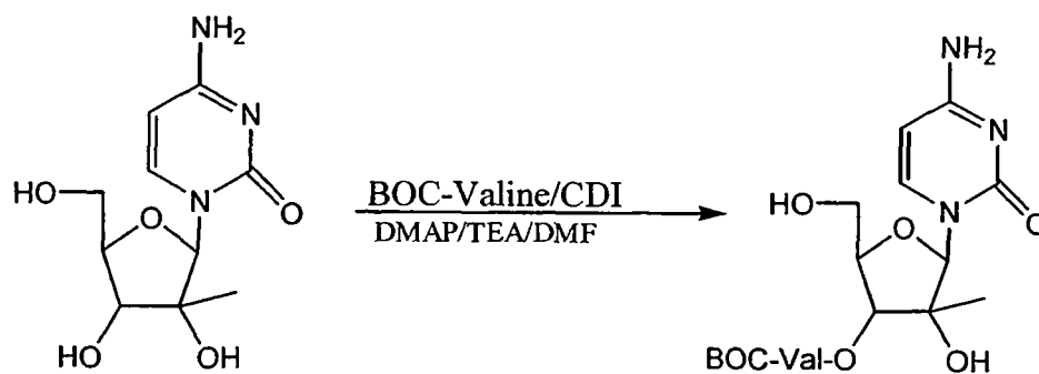
Figure 1: Direct Esterification for a Pyrimidine Nucleoside
