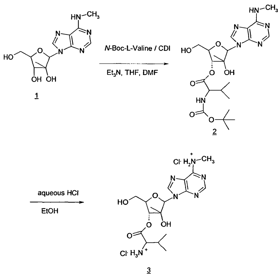
Figure 2: Direct Esterification for a Purine Nucleoside
