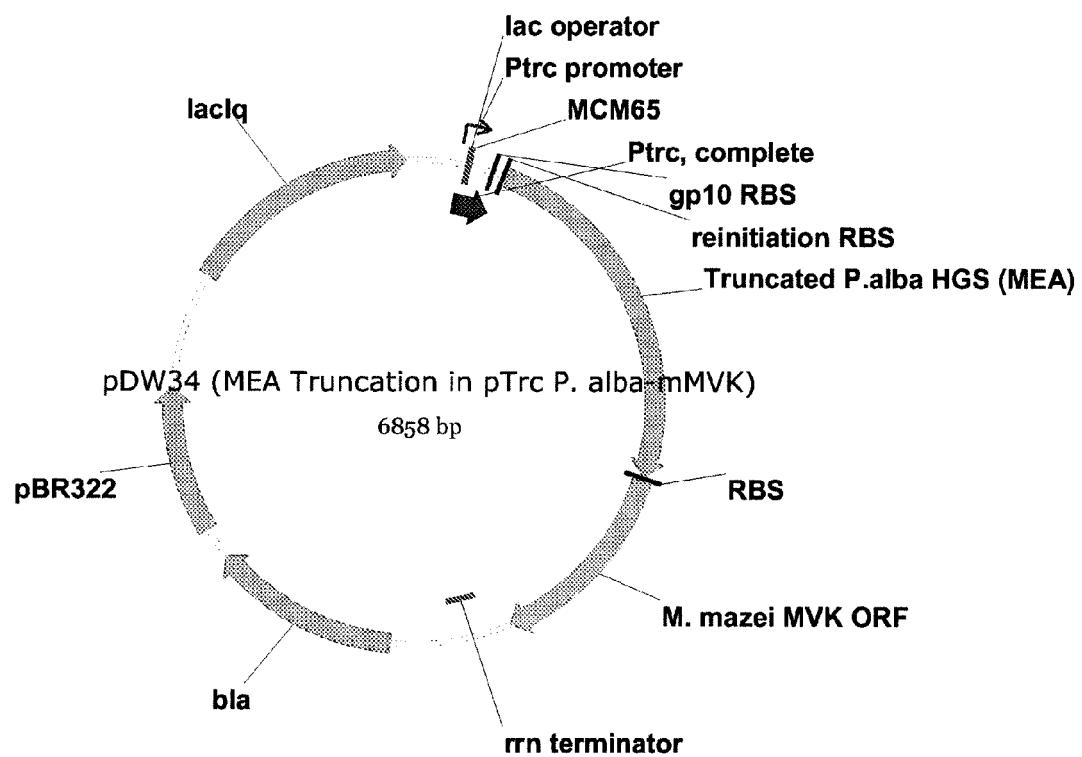
Figure 19A. Map of plasmid pDW34
