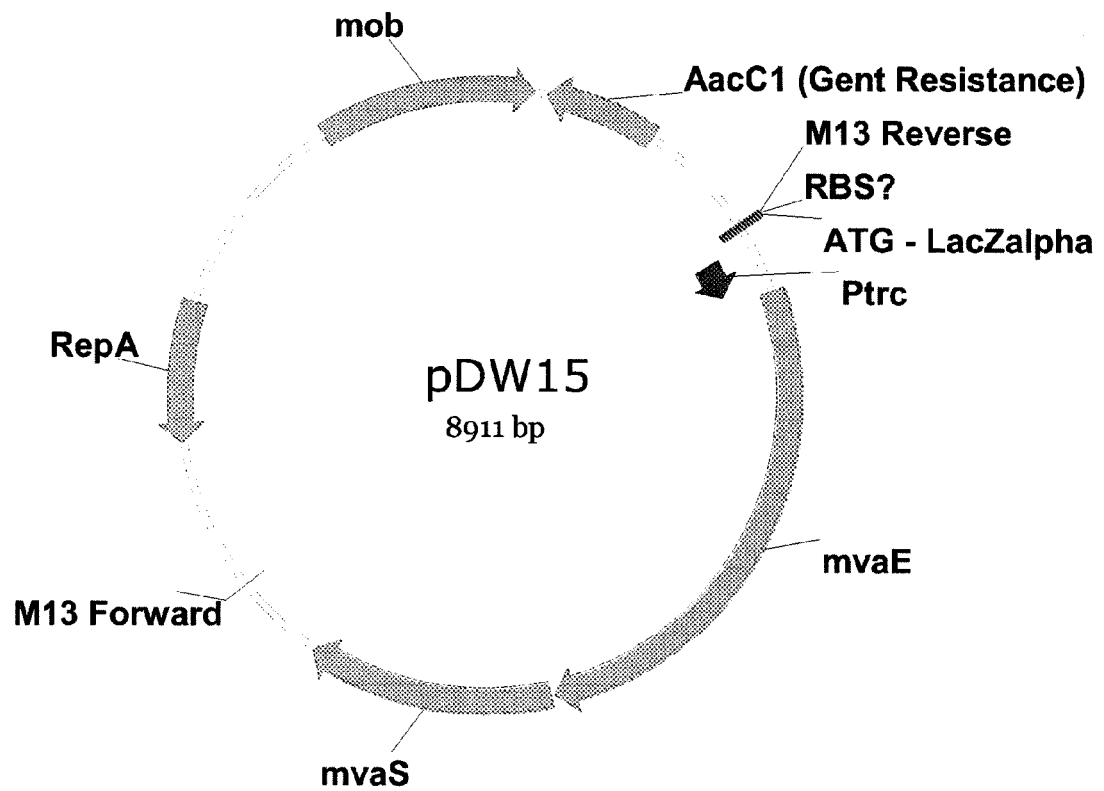
Figure 34A. Map of plasmid pDW15.
