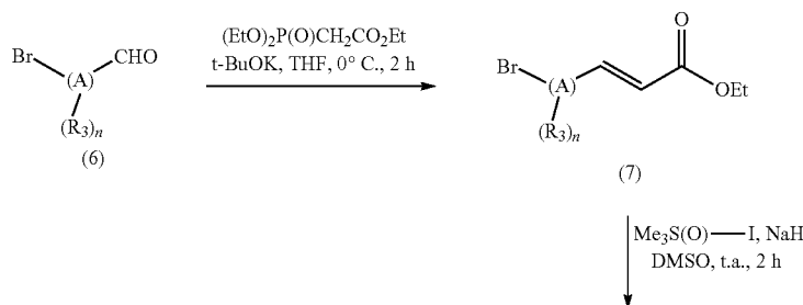
SCHEME 2: ACN (acetonitrile), DMSO (Dimethyl sulfoxide), THF (Tetrahydrofuran).
