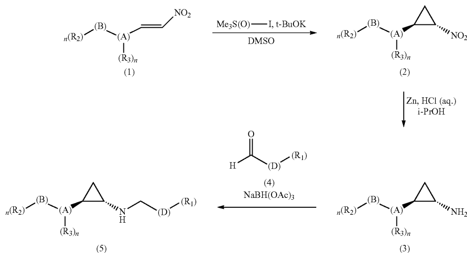
SCHEME 1: DMSO (Dimethyl sulfoxide)
