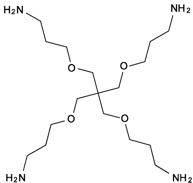
Star-PEG amine, pentaerythritol (3-aminopropyl) ether
