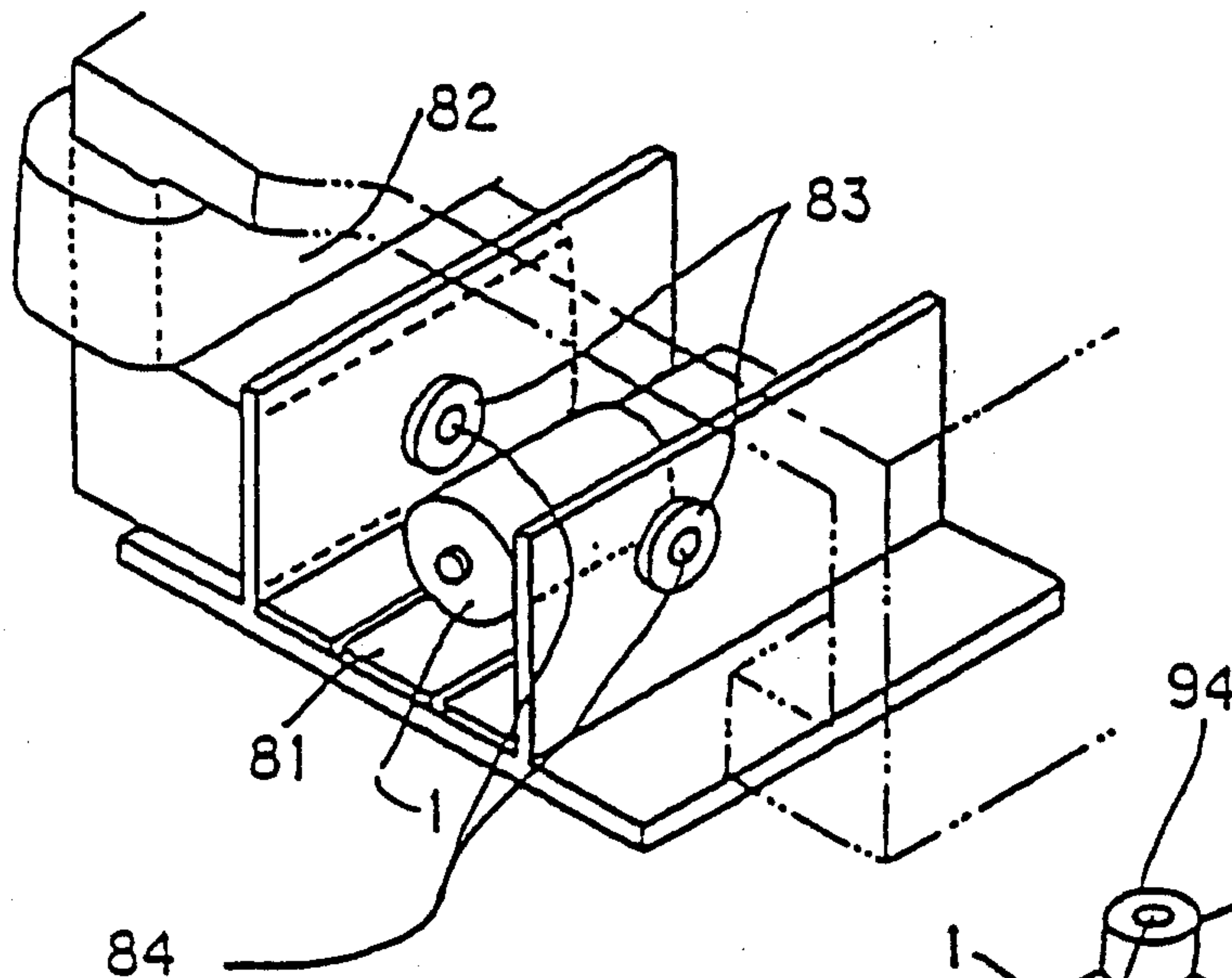
FIG. 10(b) LOCAL AC EXCITATION COIL-2
