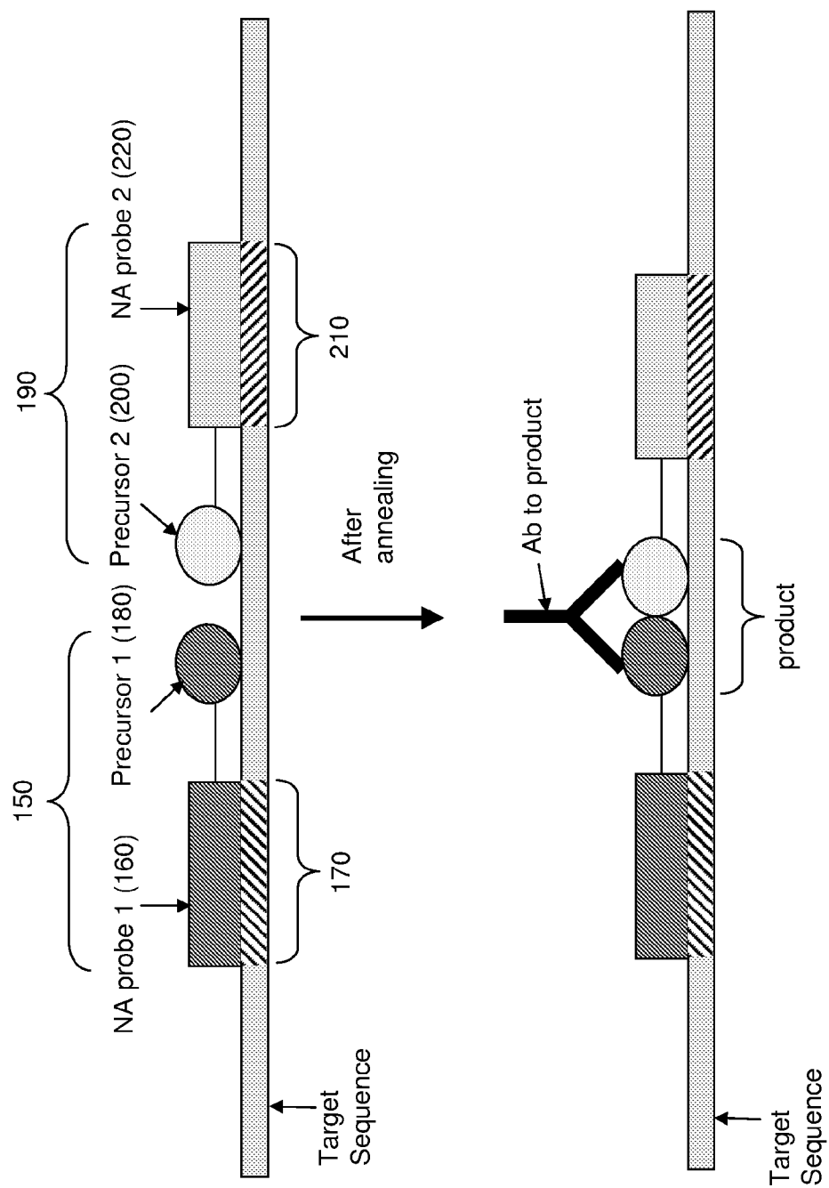
FIG. 19 – DPC DNA Sequence Detection Based upon Epitope Creation
