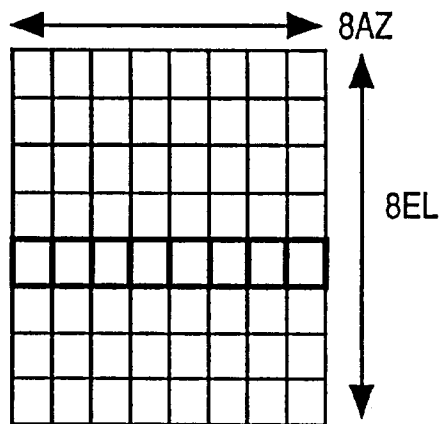
MULTIBEAM BEAMFORMER
