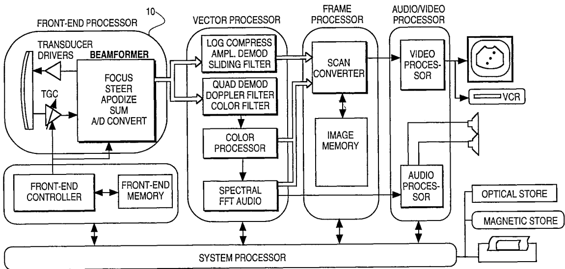
ULTRASONIC IMAGING SYSTEM BLOCK DIAGRAM
