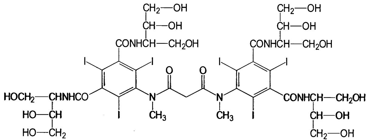
iotrolan
