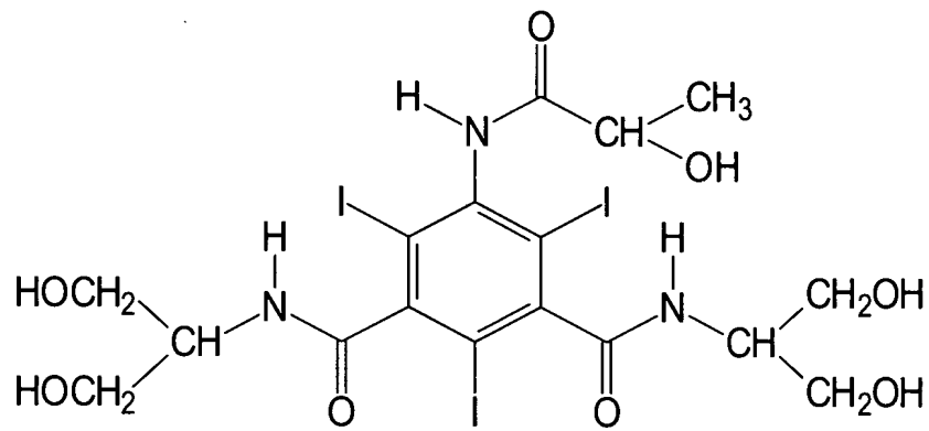
iopamidol
