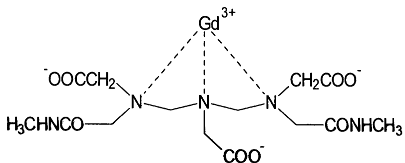
gadodiamida
