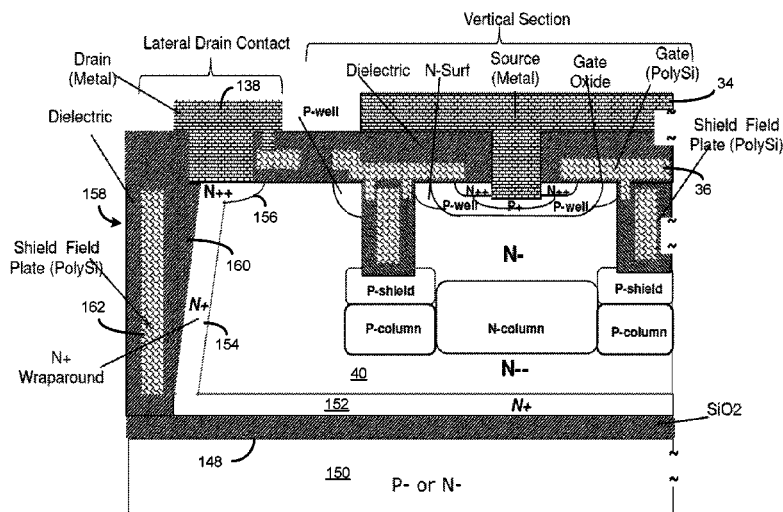
Device Structure With SOI and Surface Drain Electrode
