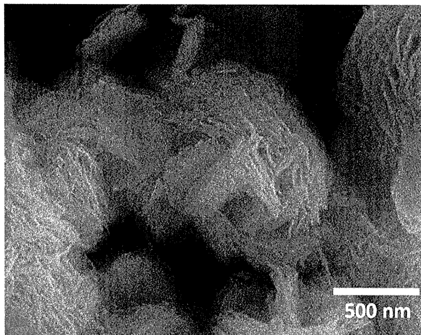
Figure 11B
