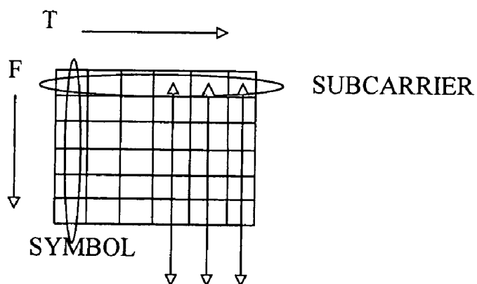
FIG 5. SUBCARRIER REFERENCE PHASE DRIFT AT EACH TIME INTERVAL IS OBTAINED BY AVERAGING VALUES DETERMINED AT ALL FREQUENCIES
