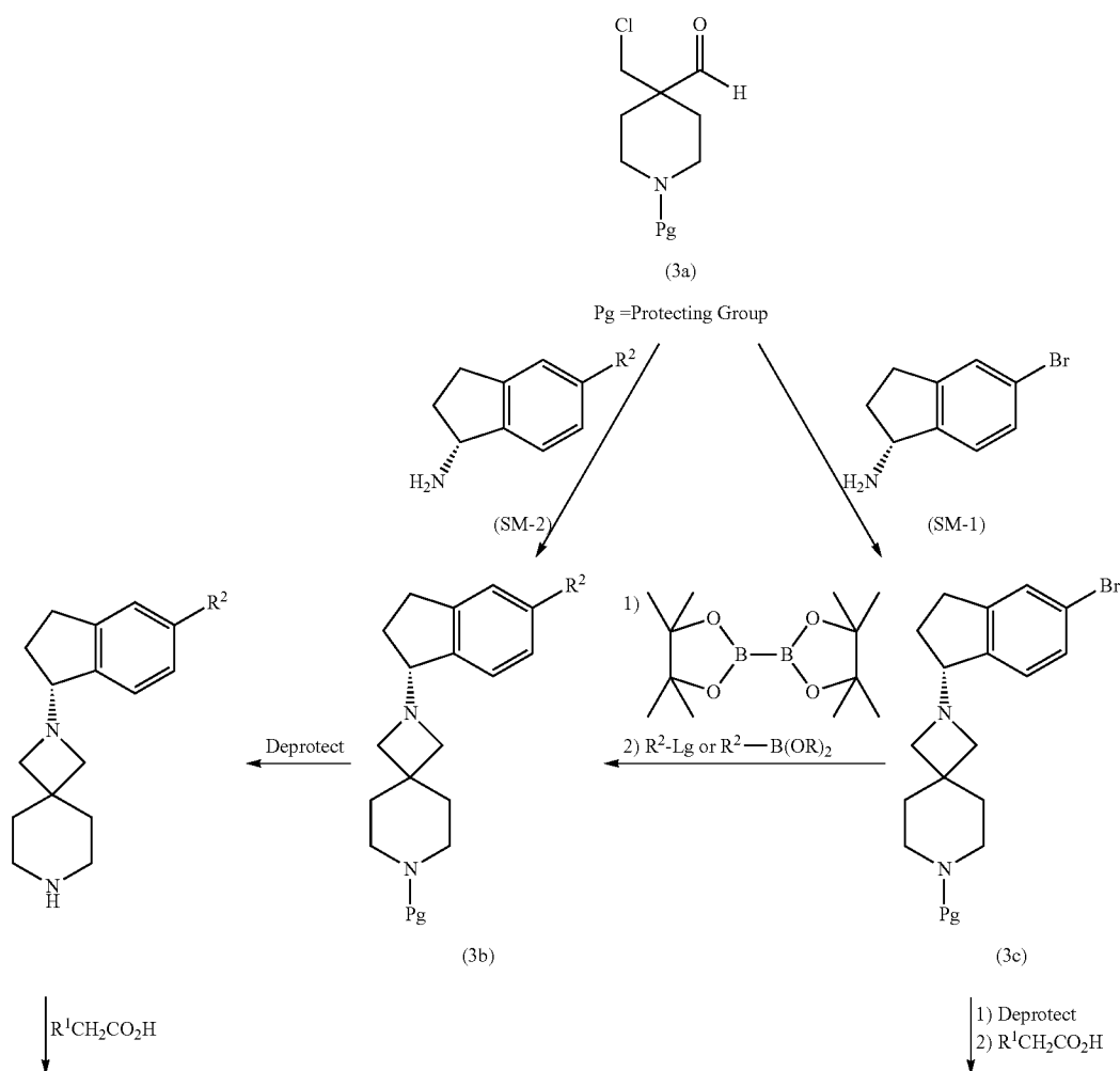
Reaction Scheme III
