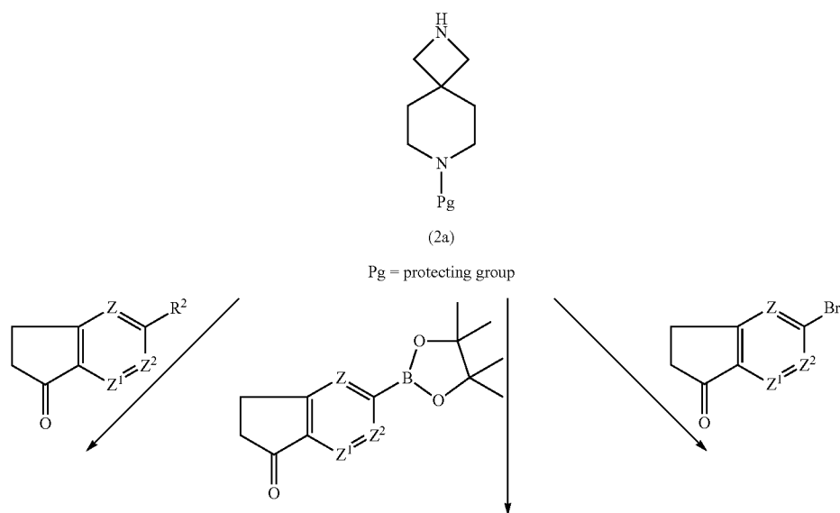
Reaction Scheme II
