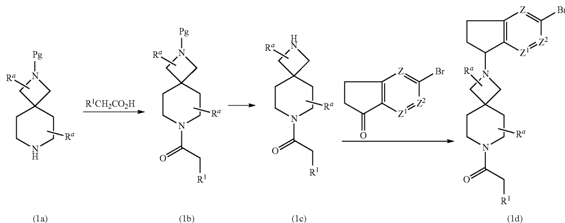
Reaction Scheme I
