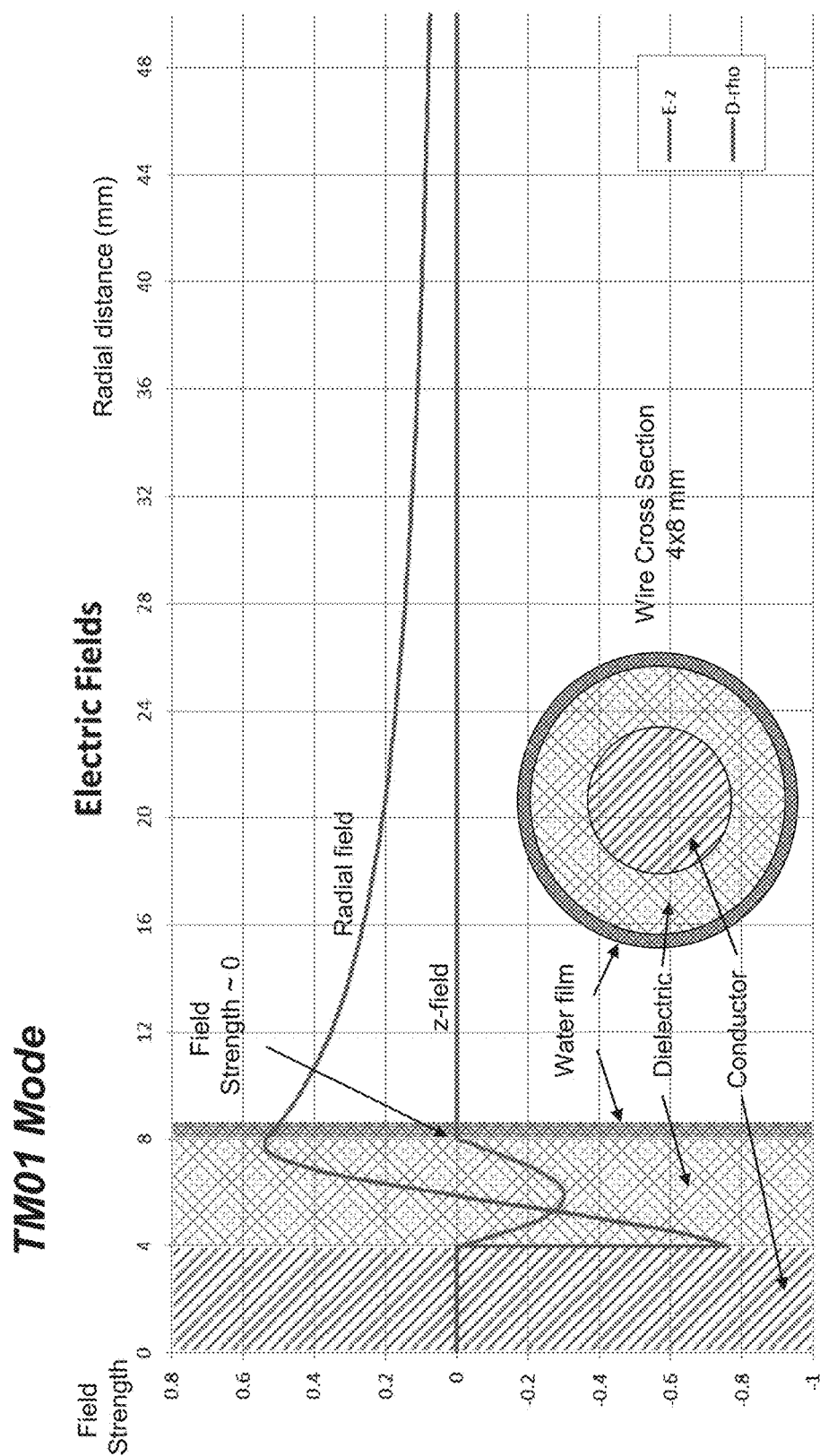
\text{TM}_{01} \quad 30.437 \text{ GHz} a = 4 \text{ mm } b = 8 \text{ mm } e_R = 2.5
