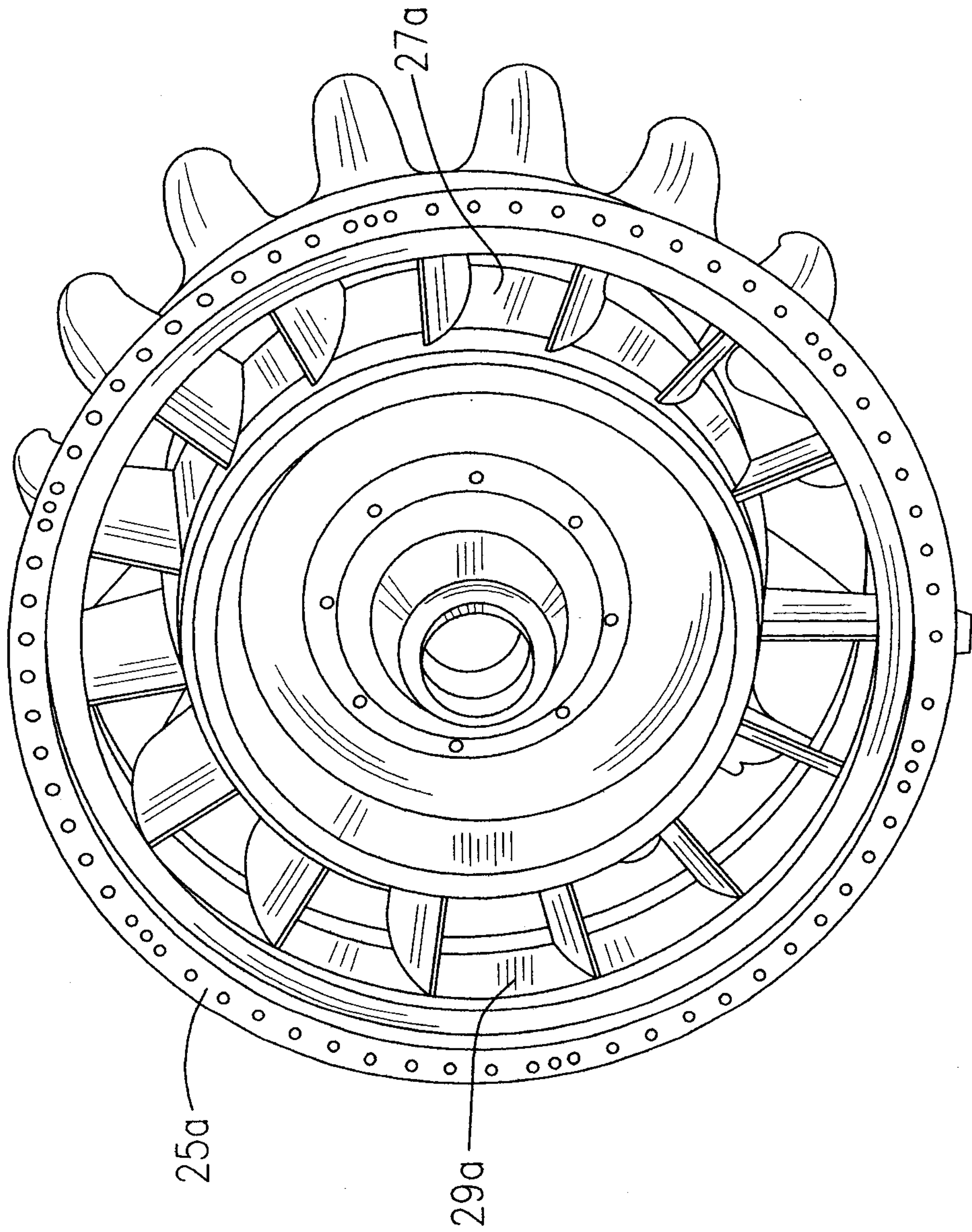
FIG. 9 PRIOR ART
