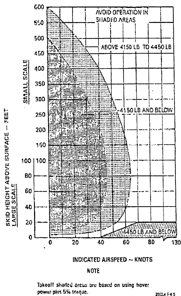
Figure 4. Height-Velocity diagram for the Bell 206L-4 Helicopter Results
