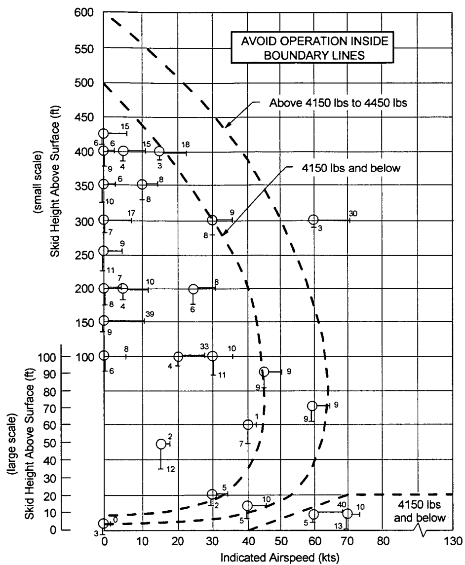
Figure 6 Touchdown ground-speed and sink-rate (light weight condition)
