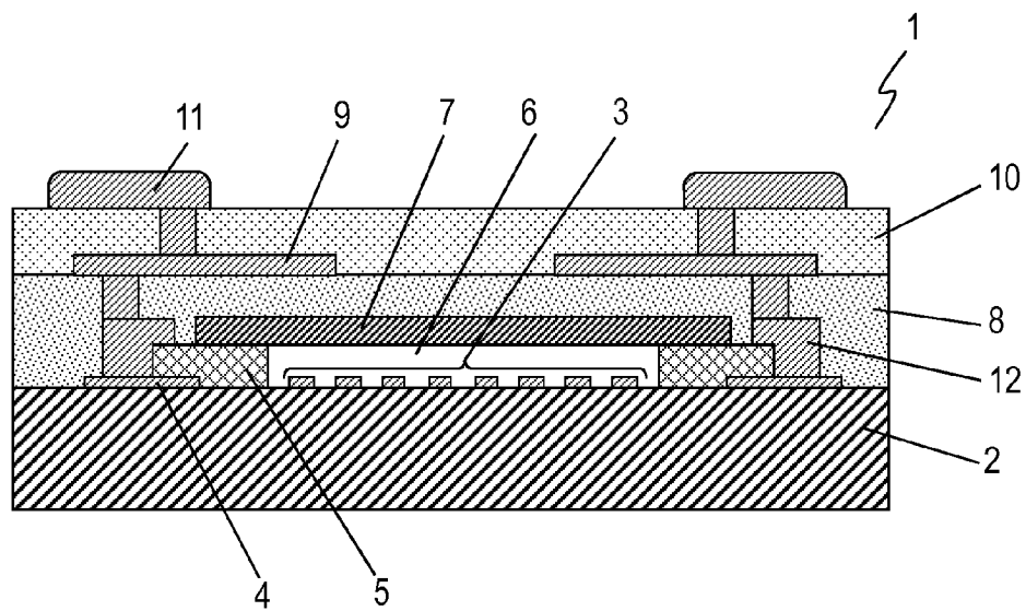
Fig. 9 PRIOR ART
