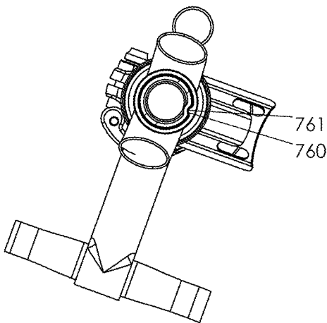
SECTION L-L
