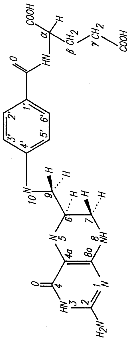
TETRAHYDROFOLIC ACID OR FH4
