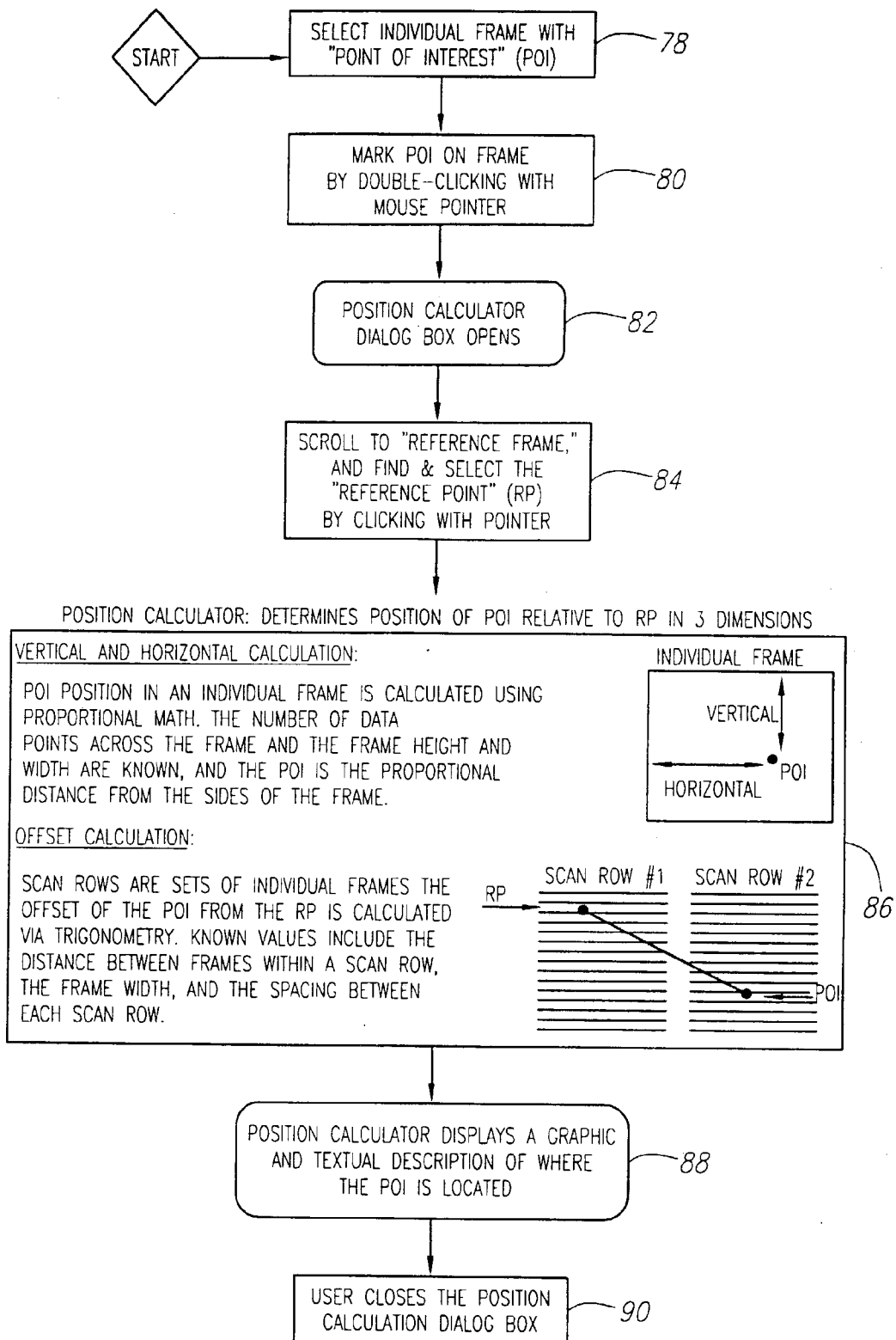
FIG. 10 POSITION CALCULATOR IN VIEWING PROGRAM
