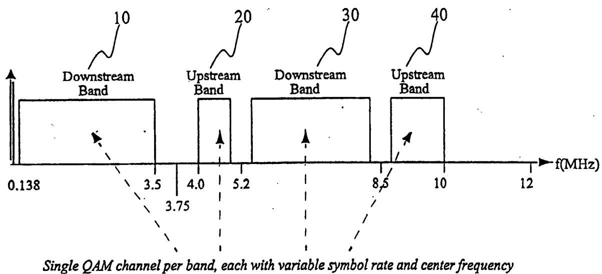
FIG. 4: Adjustment of Total Bandwidth in a SCM System
