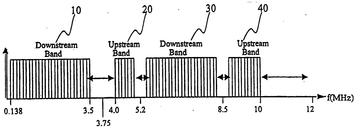
FIG. 3: Adjustment of Total Bandwidth in an MCM System
