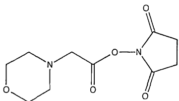
Morpholino-4-yl-acetic acid N-hydroxysuccinimide ester Molecular Weight = 242.23
