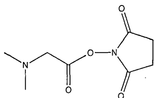
Dimethylamino-acetic acid N-hydroxysuccinimide ester Molecular Weight = 200.20
