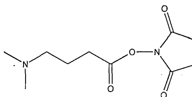
Toluene-4-sulfonate Dimethylamino-butyric acid N-hydroxysuccinimide ester Molecular Weight = 229.26
