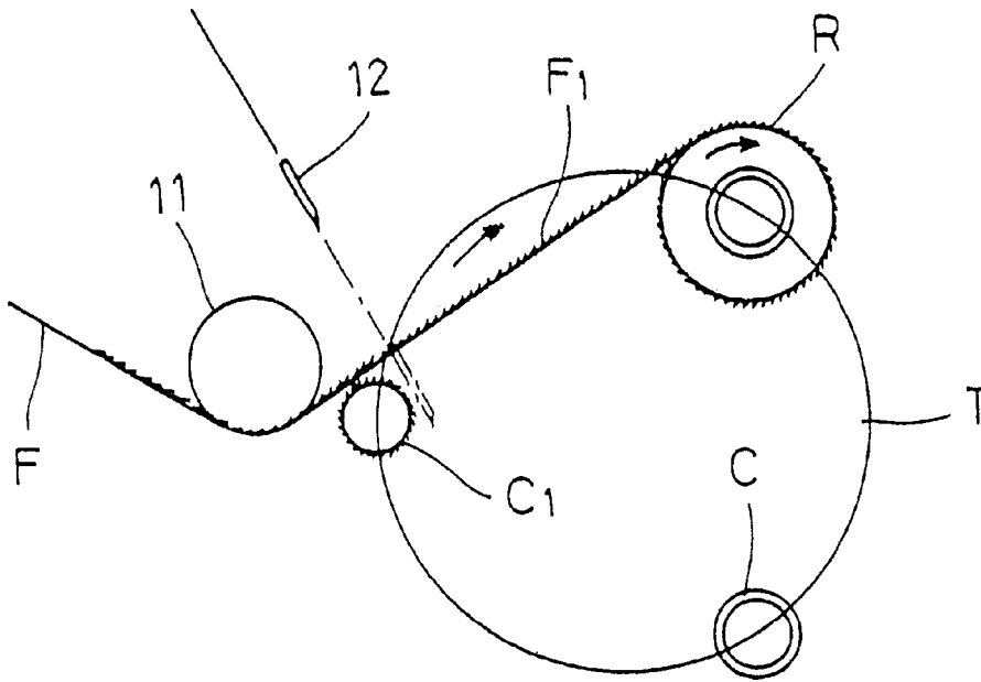
FIG. 4 PRIOR ART
