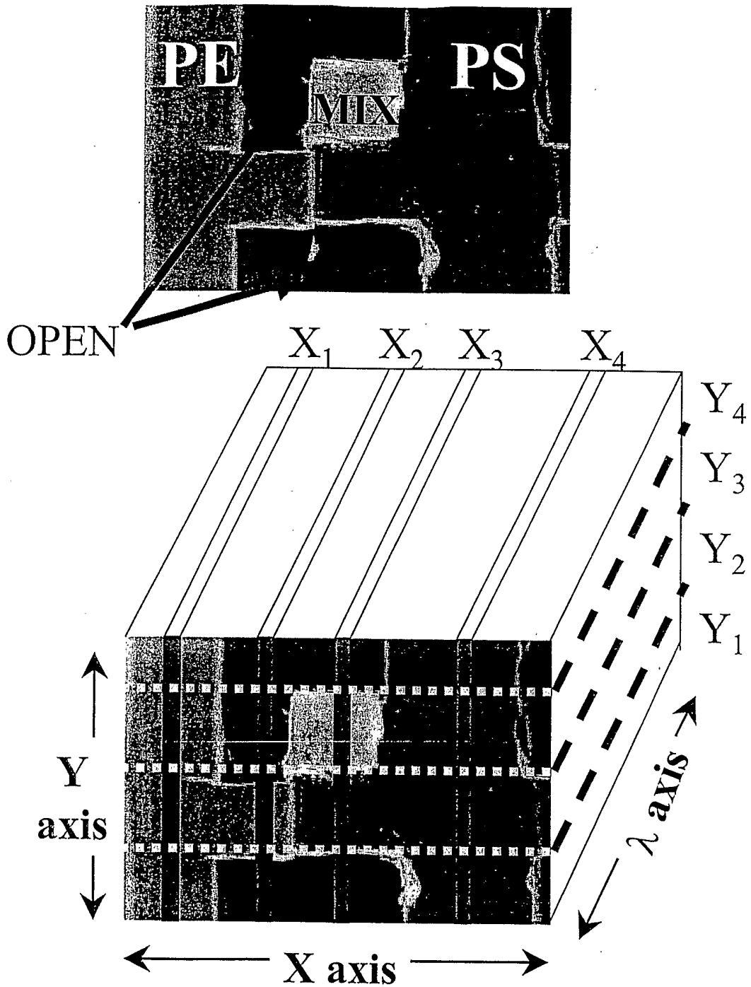
Pushbroom scan for X spatial dimension
