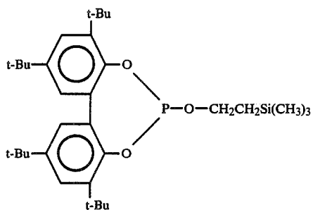
15 phenyl[3,3',5,5'-tetra-t-butyl-1,1'-biphenyl-2,2'-diyl]phosphite
