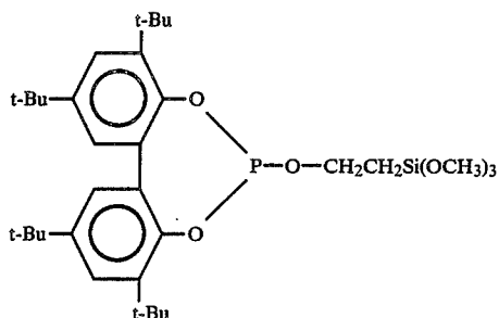
20 1,1'-binaphthyl-2,2'-diyl-(2,6-di-t-butyl-4-methylphenyl)phosphite
