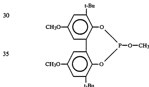
40 methyl[3,3'-di-t-butyl-5,5'-dimethoxy-1,1'-biphenyl-2,2'-diyl]phosphite
