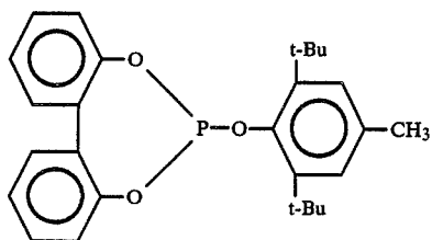
1,1'-biphenyl-2,2'-diyl-(2,6-di-t-butyl-4-methylphenyl)phosphite
