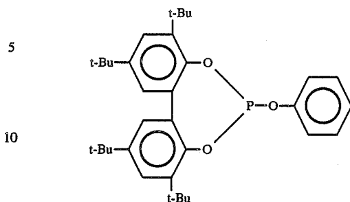
15 phenyl[3,3',5,5'-tetra-t-butyl-1,1'-biphenyl-2,2'-diyl]phosphite
