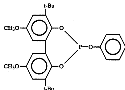
Ligand A
