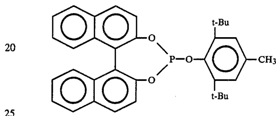
20 1,1'-binaphthyl-2,2'-diyl-(2,6-di-t-butyl-4-methylphenyl)phosphite
