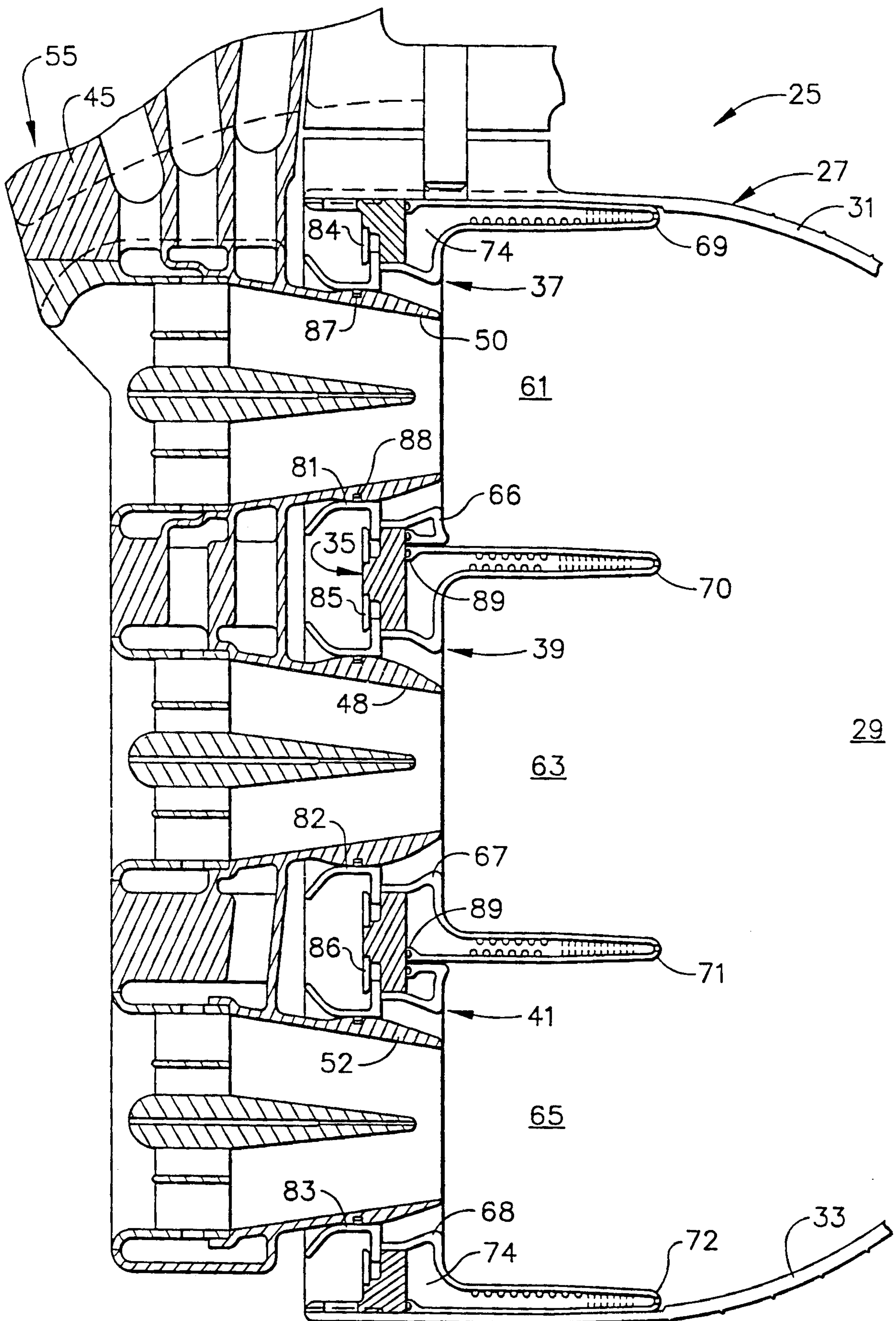
FIG. 1 (PRIOR ART)
