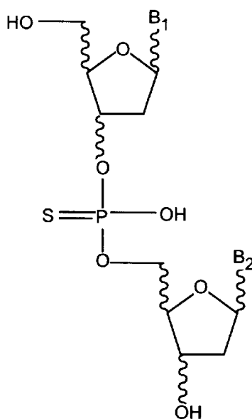
Phosphorothioates
