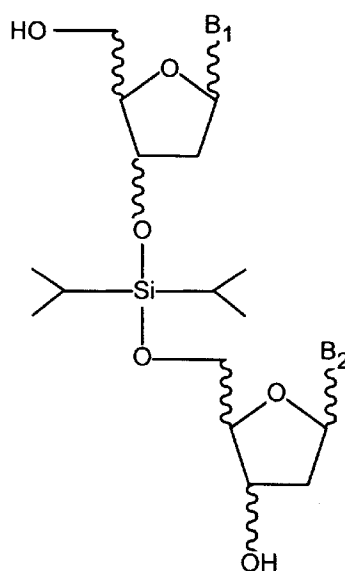
Silyl Ethers
