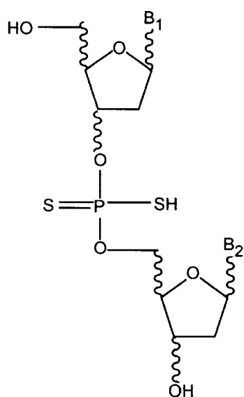
Phosphorodithioates
