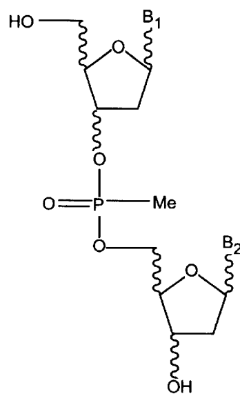
Methyl phosphonates
