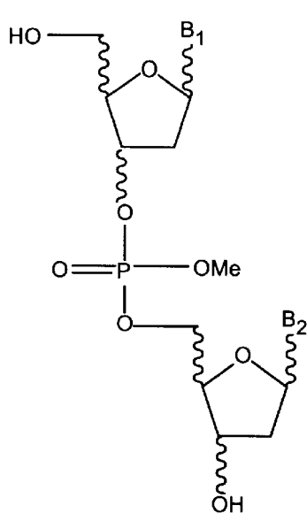
Methox phosphotriesters
