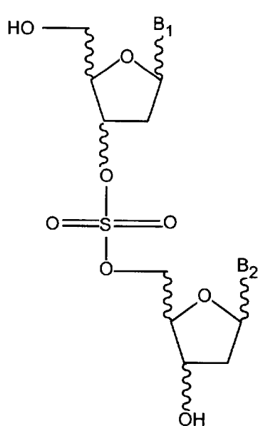
Sulfonates
