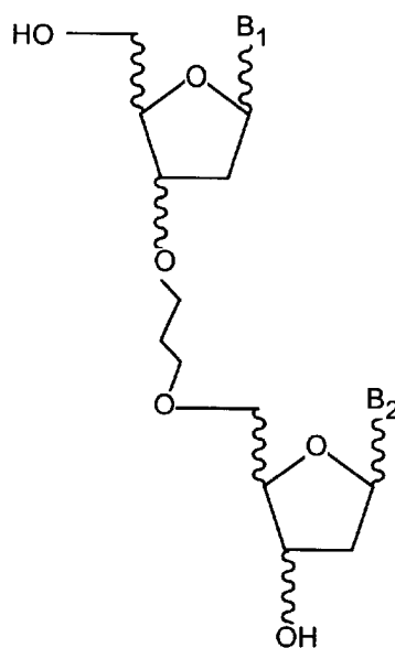
Ethylenedioxy ethers
